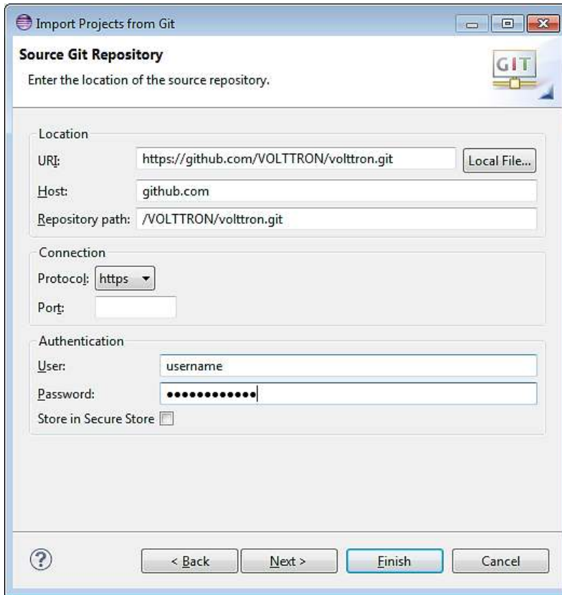
Figure 39: Checking Out Transactional Network with Eclipse (continued)
