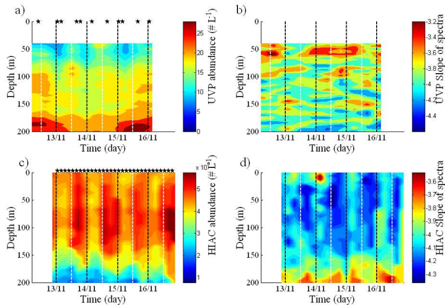
Fig. 4. Temporal distribution of the total particle abundance at the GYR site of the UVP ( a ) and HIAC ( c ) and particle slope of size spectra of the UVP ( b ) and HIAC ( d ). The black dashed lines indicate local mid-night time while the white dashed lines indicate local mid-day time. The sampling is indicated by the stars.
