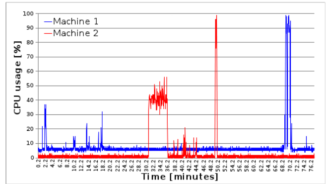
Fig. 1. CPU usage by VBS client on two computers
