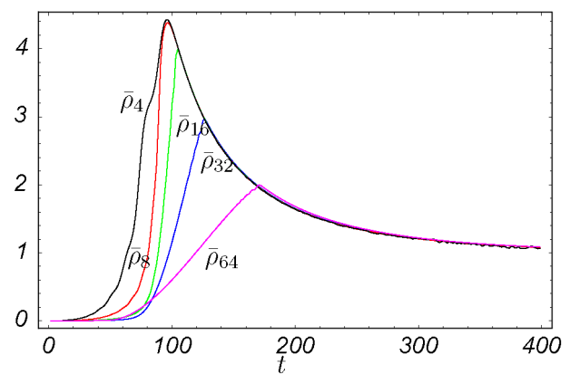
FIG. 2 (color online). The plots of the average density as function of time for various radii of spheres over which the averaging is performed. The initial radius of the cavity in this case is a = 128 . The radii of averaging spheres are b = 4, 8, 16, 32, 64 . The average density is calculated as \bar{\rho}_b = 3 \int_0^b \rho(r) r^2 dr / b^3 .
