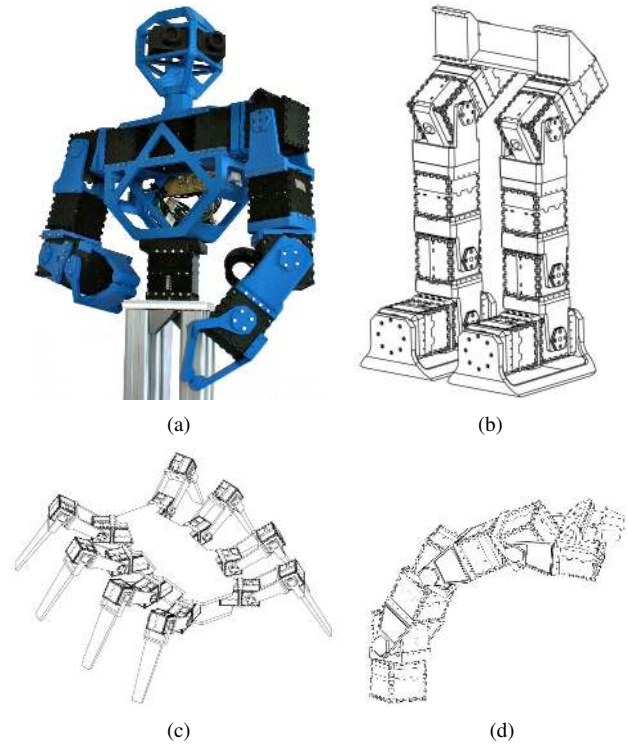
Fig. 10. Examples of possible robotic systems that can be built. In (a) the realised upper body is shown, in (b) a pair of 6 DOFs legs, in (c) a spider and in (d) a seven degrees of freedom arm.
