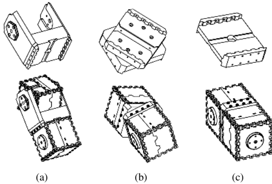
Fig. 9. The three possible types of connections that can be used to realize a robotics system. (a) and (b) show two kinds of revolute joints, with respectively, perpendicular and parallel axis. (c) shows the rigid connection.
