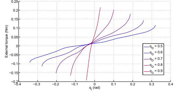
Fig. 12. Average torque vs displacement plot, for VSA II. The relationship between the link displacement and the reaction-force is evident in the figure. The asymmetrical behaviour is due to imperfect matching between the springs in the prototype.
