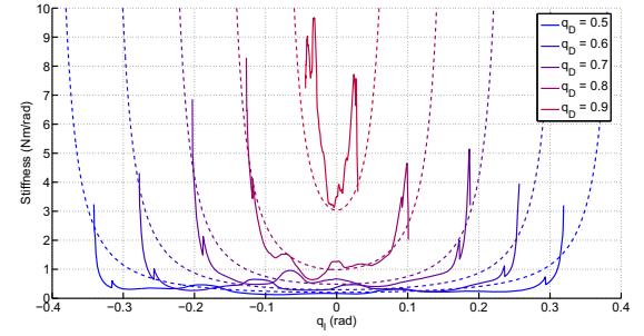
Fig. 13. Stiffness vs displacement plot, theoretical (dashed) and experimental (solid). Larger differential angles make the mechanism stiffer.
