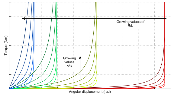
Fig. 3. Theoretical torque deflection characteristics can be obtained with various values of R/L and k for \theta \geq 0 (curves are symmetric with respect to the origin). The effect of k is to scale the overall function. Graphs are plotted for k = 20, 40, 80, 160, 320 Nm/rad.
