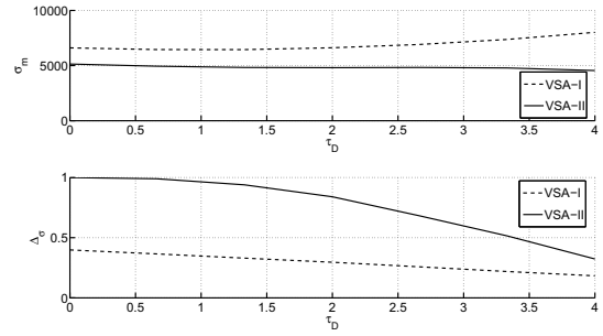
Fig. 8. Trends of \sigma_m and \Delta_\sigma , for VSA-I and II obtained from data in Fig.7.
