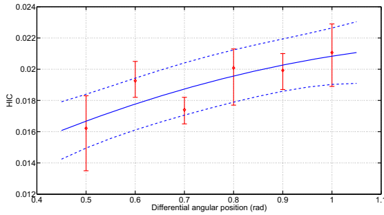
Fig. 14. Experimental values HIC vs differential angular position, with fitting polynomial. Lower values of stiffness, tend to get lower values of HIC and so are safer.
