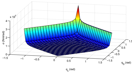
Fig. 6. VSA-I stiffness for joint shaft position q_l = 0 varying q_S and q_D in the admissible range. q_S and q_D have similar definitions.
