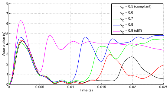
Fig. 15. Acceleration of the impacted body during different impact test with different stiffness levels, it can be noticed the separation between the contribution to the impact due to the link mass (the first peak of the profiles) and the contribution due to the motor and gears inertia (the second peak, which happens later in time for compliant configurations and sooner for stiff configurations).
