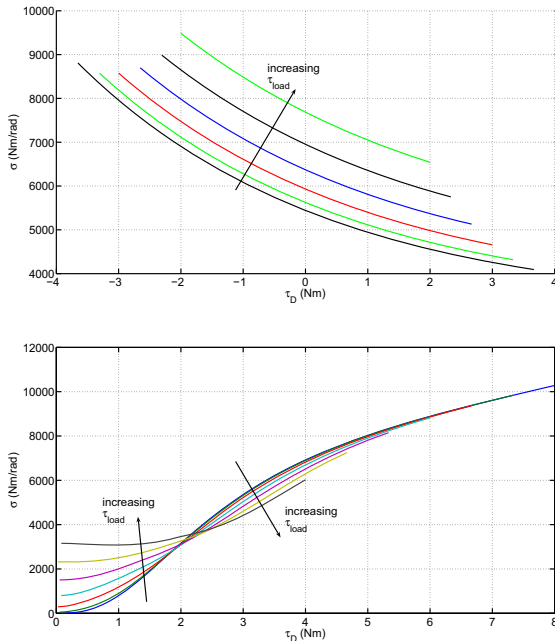
Fig. 7. Stiffness - torque relationship for VSA-I (top) and VSA-II (bottom). The plots show the stiffness seen from the link as a function of the differential torque \tau_D , for increasing values of external disturbance torque on the link \tau_{load} . Curves are obtained with limited torque \tau_{MAX} = 4.356 for the motors, and external load torque \tau_D = \{0, 0.66, 1.33, 2, 2.66, 3.33, 4\} .
