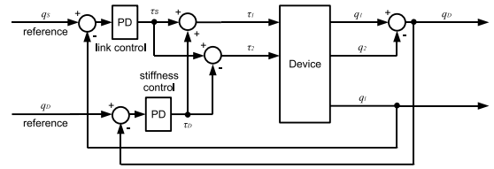
Fig. 5. Control scheme used.
