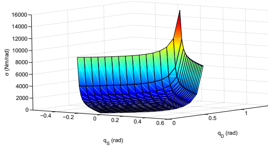
Fig. 4. VSA-II stiffness for joint shaft position q_l = 0 varying q_S and q_D in the admissible range.
