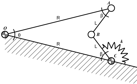
Fig. 2. Line diagram of 4-bar transmission mechanism of VSA II. Link \overline{OA} of length R is driven by a motor at O . The torque spring k has a linear behaviour. Stiffness seen at O attains non-linearity through the geometry, where angle \theta at O and transmission angle \beta are related non-linearly.
