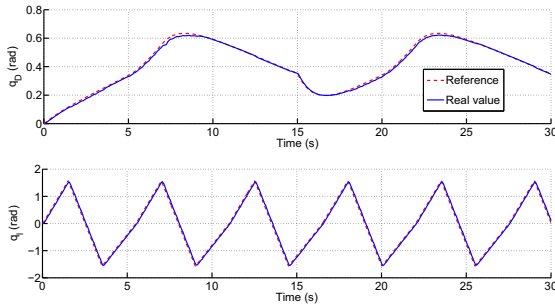
Fig. 11. Trajectory following with the implemented PD control system (reference dashed, trajectory solid).
