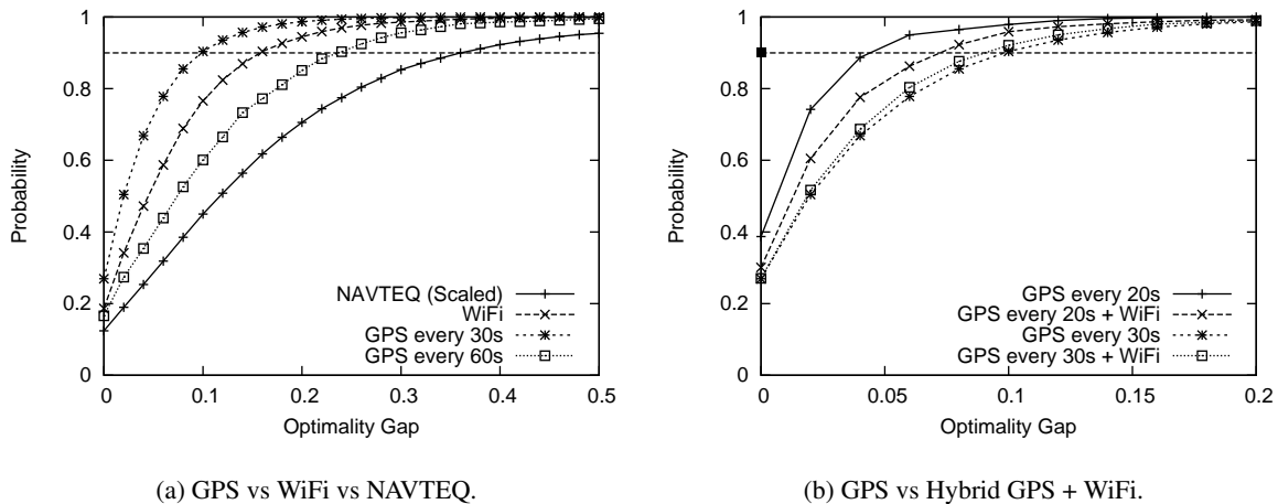
Figure 8: CDF of Optimality Gap when route planning using VTrack. Larger optimality gaps are worse.
