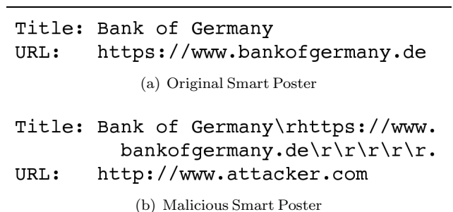
Figure 1. URL Spoofing
