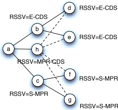
Figure 2. Relay set selection considering RSSV: Router a makes the decision based on the RSSV declared by TLVs.
