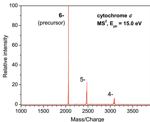
Figure 3 Mass spectrum of the product ion resulting from photodetachment of the 6^- precursor cytochrome c ion at 15 eV. The precursor ion was isolated, stored in the ion trap and irradiated for 200 ms.
