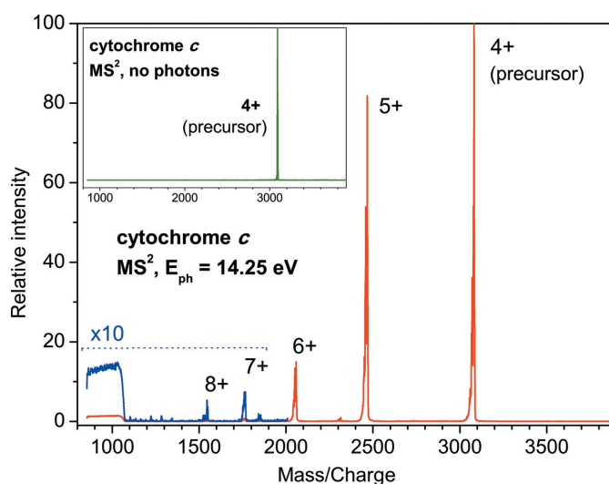
Figure 2 Mass spectrum of the product ion resulting from photoionization of the 4 + precursor cytochrome c ion at 14.2 eV. The precursor ion was isolated, stored in the ion trap and irradiated for 600 ms.
