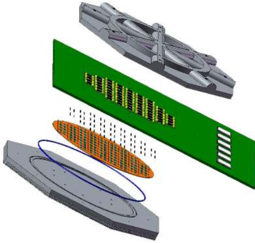
Fig. 1. A FACETS -wafer with motherboard and mounting bracket. From top to bottom: top mounting bracket, motherboard containing digital network chips, FPGAs and passive components, elastomeric connectors, silicon wafer with analog network chips, seal ring, bottom mounting bracket.
