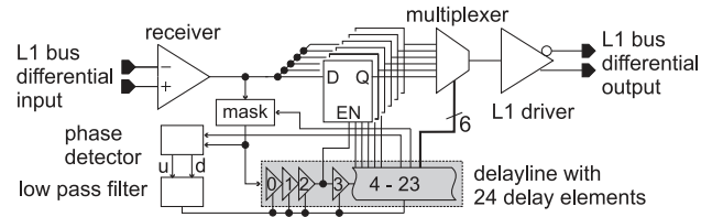
Fig. 8. Schematic diagram of a repeater. A 24-tap DLL locks on the input frame and acts as timing reference for the multiplexer which generates the serial output stream.
