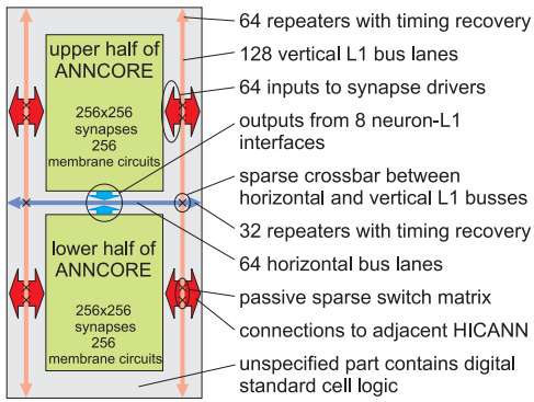
Fig. 3. Block diagram of a HICANN chip.
