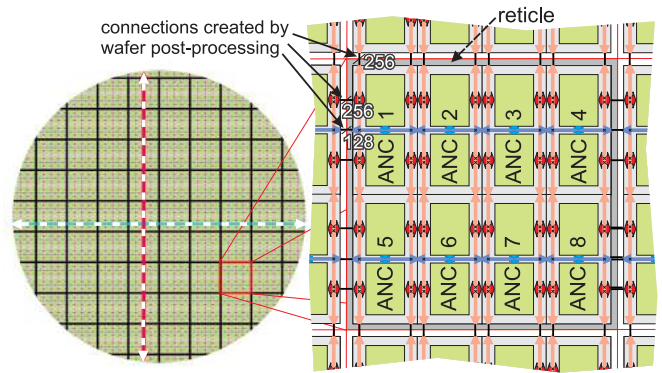
Fig. 2. A FACETS -Wafer containing 56 complete reticles. The dashed arrows depict one bundle of horizontal respectively vertical inter-neuron connections. A single reticle is enlarged showing the arrangement of the analog neural network chips (ANC). The number of wires is given for each type of connection created by wafer post-processing.
