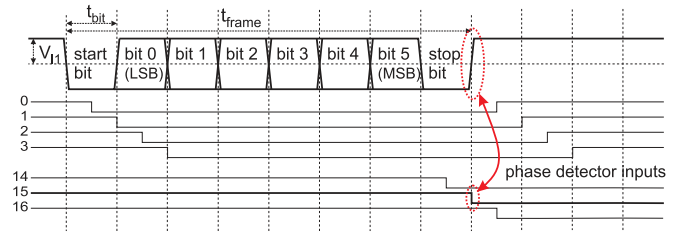
Fig. 6. Timing of a serial L1 data frame. Shown is the differential signal V_{11,\text{pos}} - V_{11,\text{neg}} . The output signals of the delay-locked loop (DLL) used for timing recovery are shown beneath. If the falling-edge of output 15 is aligned with the rising edge of the L1 signal, the DLL is locked.
