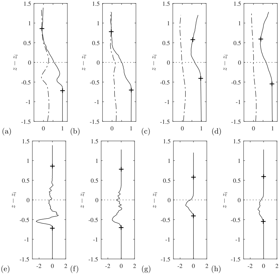
FIGURE 11. Ship centerline wake profiles at select locations as a function of z - z_i , where z_i is the location of \bar{\rho} = 0.5 . (a-d) — \bar{u}(z) ; - - \bar{w}(z) ; and + \bar{\rho} = (0.01, 0.99) . (e-h) — \bar{\rho}\bar{\omega}_y and + \bar{\rho} = (0.01, 0.99) . (a,e) case B \bar{x}=1 ; (b,f) case C \bar{x}=1 ; (c,g) case B \bar{x}=3 ; (d,h) case C \bar{x}=2.1 .
