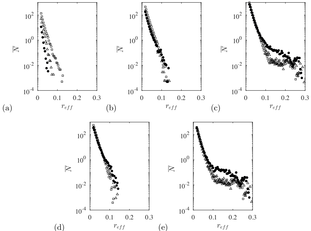
FIGURE 14. Average cavity density spectra as a function of effective radius \bar{N}(r_{\text{eff}}) for all three cases: \bullet case A; \triangle case B; and \square case C. (a) CCW x < x_c ; (b) RT x_c < x < x_B ; (c) DW for x > x_B ; (d) DW for |y| \leq B ; and (e) DW |y| \geq B . x_B defined in table 2. Data normalized by each measurement volume \forall_i and cavities with r_{\text{eff}} < a_N not shown.
