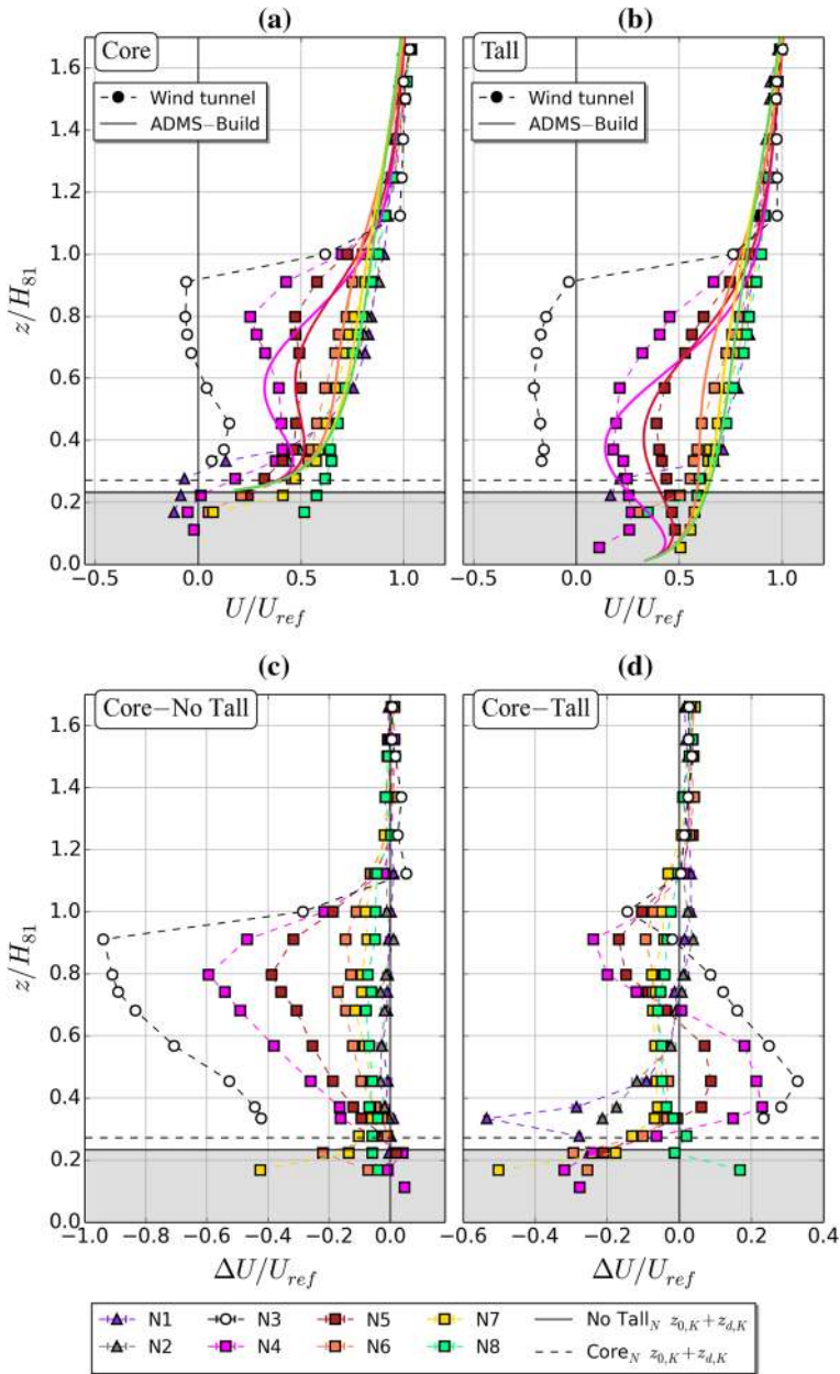
Fig. 4 Vertical profiles of U for sites on a longitudinal transect through building T_{81} (north orientation) for the, a Core, and b Tall cases; and profiles of the velocity difference \Delta U (note different x -axis scales) for c Core-No Tall, and d Core-Tall (site codes in Fig. 2c). Wind-tunnel data shown as symbols. Triangle: site upwind of the tall building, circle: near-wake site, square: main-wake site. ADMS-Build model results (thick solid lines) in the main wake shown in (a, b). Shading indicates H_{ave} + \sigma_H for No Tall N (Table 3)
