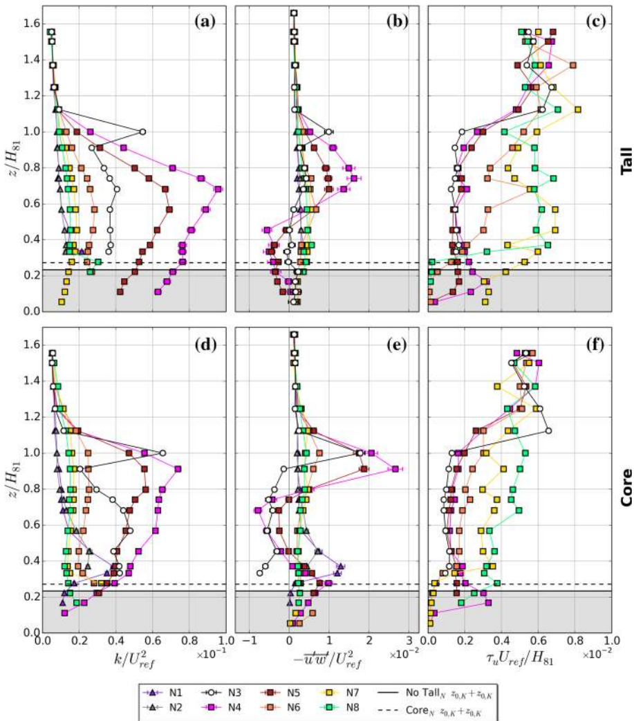
Fig. 8 Vertical profiles of a, d turbulence kinetic energy, b, e vertical turbulent momentum flux, and c, f turbulence integral time scales of the u -component on a longitudinal transect through building T_{81} (north orientation) in the a–c Tall and d–f Core set-ups. Symbols as in Fig. 4
