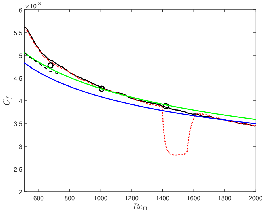
Fig. 1 Color online. Skin friction coefficient C_f from present DNS (reference cases in black): (—) case 3, (— · —) cases 1 and 2; circles represent C_f from Ref. [32]; green (light grey) line is the low Reynolds number empirical profile [39], while the blue line (dark grey) is the high Reynolds number empirical profile [22]; dotted red line is the friction coefficient for case 3 with wall oscillation.
