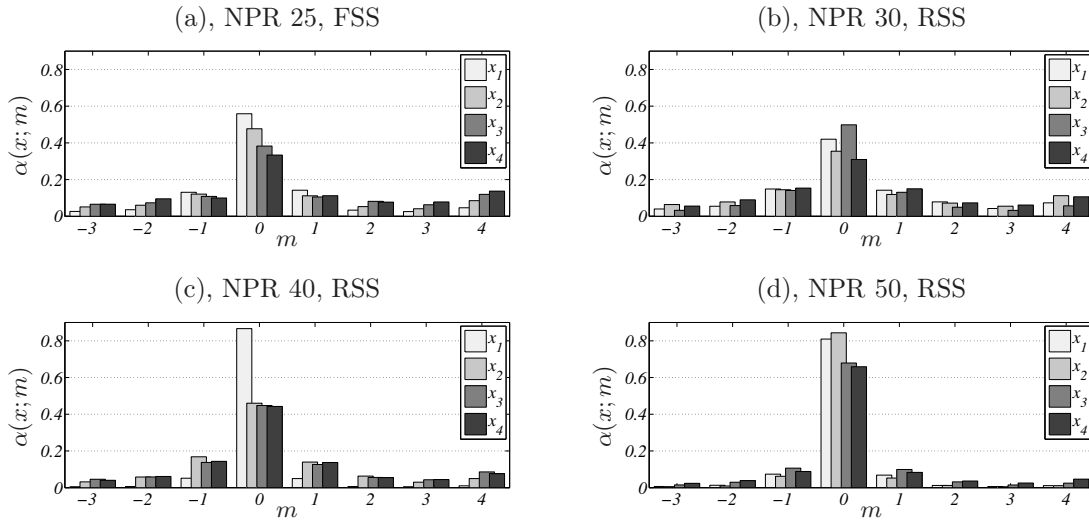
Fig. 12 Scaled eigenspectra of the azimuthal Fourier modes.
