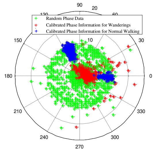
Figure 10 - Calibrated phase information for the wandering behaviors and the normal walking behavior
