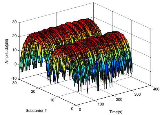
(a). Variations of amplitude information for 30 subcarriers
