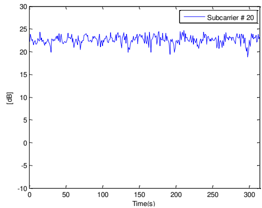
(b). Variances of amplitude information for an individual subcarrier
