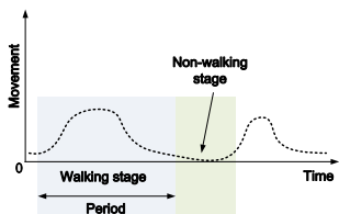
Figure 2 – Spatio-temporal movement
