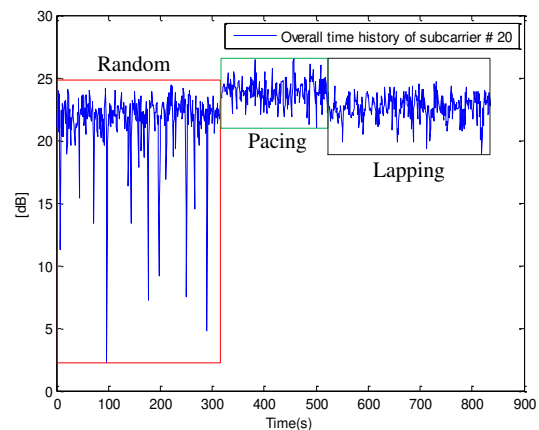
Figure 7 – Combined time history of lapping, pacing and wandering randomly
