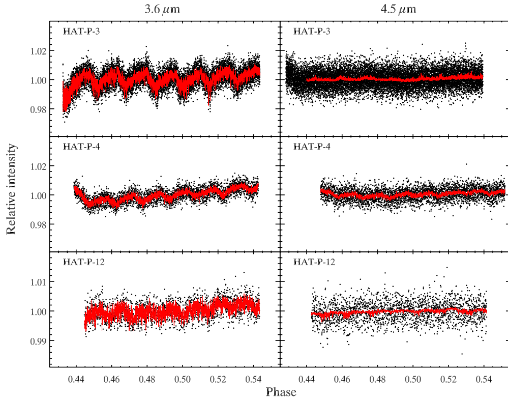
Figure 1. The uncorrected time series photometry for HAT-P-3, HAT-P-4 and HAT-P-12 at 3.6 and 4.5 \mu\text{m} during secondary eclipse (dots), with the best fit eclipse model we obtain (red lines). These models include the astrophysical eclipse and the instrumental effects: a linear ramp and the dependence of the measured intensity on the x - and y -position of the stellar image on the detector. All photometric points are shown here, including the initial 49 minutes of HAT-P-3 photometry, which we later reject. The best fit models only cover data that we have adopted for the fits. We discuss the data models in detail in Section 3.2. The HAT-P-12 photometry is shown on a smaller scale, since these data have the longest exposure time, and therefore the highest signal to noise per point. We do not detect the secondary eclipses of HAT-P-12b, and in these panels their depths are set to zero.
