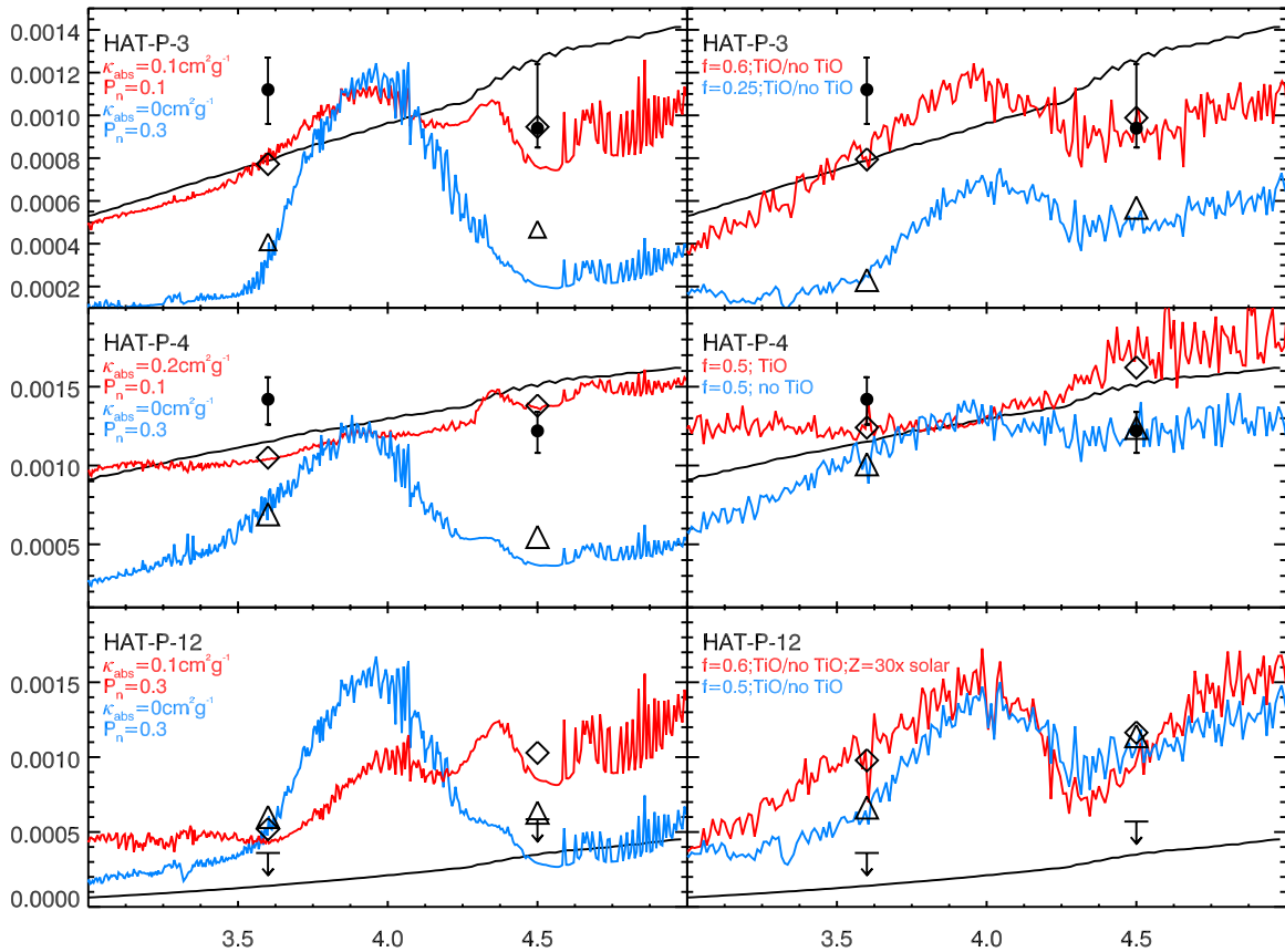
Figure 5. The measured eclipse amplitudes as a function of wavelengths (filled circles) compared to different atmospheric models: a blackbody planet with a Kurucz model for the spectrum of the star (black lines; Kurucz 1979), Burrows planetary atmospheric models (left panels; Burrows et al. 2007, 2008), and similar atmospheric models by Fortney et al. (right panels; 2005, 2006a, 2006b, 2008). The downward arrows represent 3\sigma upper limits for the HAT-P-12b eclipse depths. We have assumed effective stellar temperatures for HAT-P-3 from Chan et al. (2011) and from Knutson et al. (2010) for HAT-P-4 and HAT-P-12. Left panels: the red lines represent the inverted models, with absorption coefficient of the unknown absorber in the upper atmosphere \kappa_{\text{abs}} = 0.1, 0.2, and 0.1 \text{ cm}^2 \text{ g}^{-1} and heat redistribution parameter P_n = 0.1, 0.1, and 0.3 for HAT-P-3b, HAT-P-4b and HAT-P-12b, respectively. The blue lines are models with no inversion ( \kappa_{\text{abs}} = 0 \text{ cm}^2 \text{ g}^{-1} ) and P_n = 0.3 for all three planets. We over-plot the theoretical eclipse depths resulting from integrating the model stellar and planetary fluxes over the IRAC pass bands (diamonds for the inverted models and triangles for the inverted ones). Right panels: in the Fortney model paradigm, where the stratospheric absorbers are assumed to be TiO and VO, HAT-P-3b and HAT-P-12b are sufficiently cool, so that the inverted and non-inverted (i.e., containing or not TiO and VO in the upper layers of the atmosphere) models are indistinguishable, due to TiO and VO condensation and rain-out. For HAT-P-3b, we show models with f = 0.6 (red line) and f = 0.25 (blue line); for HAT-P-4b, both models shown have f = 0.5 , but the red model has TiO in the upper layers of the atmosphere, while the blue one does not. For HAT-P-12b, the red line represents a model with f = 0.6 , while the blue line shows a model with f = 0.5 . All Fortney model atmospheres have solar composition, except the red model for HAT-P-12, which has metallicity 30 times higher than solar. For a more detailed explanation on the models see Section 4.1.
