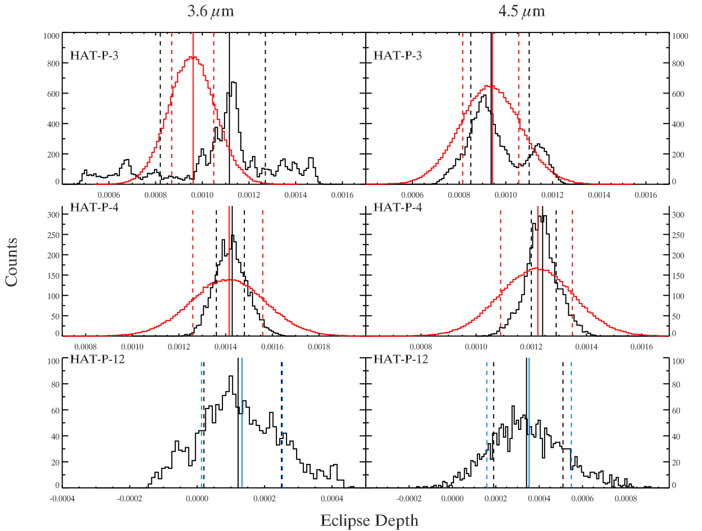
Figure 4. We show the histograms of eclipse depth values that result from the prayer-bead technique (black) and the MCMC iterations (red). The vertical solid lines indicate the best values from the PBMC (black), MCMC (red), and linear regression (blue), which we take to be the median of the eclipse depth values of the prayer-bead and MCMC runs. The dashed lines bracket the regions centered on the medians that contain 68% of the recorded values for prayer-bead (black) and MCMC (red). Since MCMC and PBMC address different noise effects, we adopt as final best values and uncertainties the results from the technique which yields the larger uncertainty region. For HAT-P-12, since there is no secondary eclipse detected, the MCMC does not converge and the prayer-bead is performed with the central phase fixed at 0.50007. The blue dashed lines indicate the 1\sigma estimates, based on the linear regression used to determine the eclipse depth in the original data sets. We conservatively adopt these as final best values since they are larger than the prayer-bead uncertainties.
