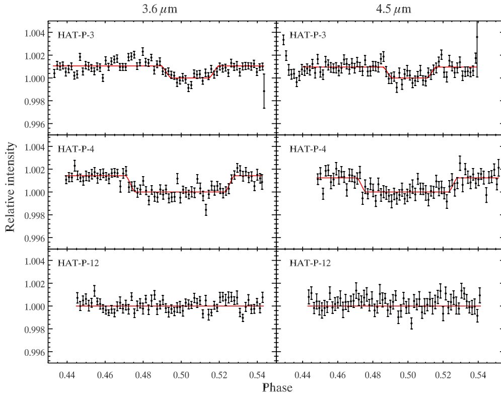
Figure 3. The binned time series photometry for HAT-P-3, HAT-P-4 and HAT-P-12 at 3.6 and 4.5 \mu\text{m} during secondary eclipse after correction for instrumental effects (dots). The bin width is 0.0015 in units of orbital phase, corresponding to about 6 minutes 16 s (HAT-P-3b), 6 minutes 36 s (HAT-P-4b) and 6 minutes 56 s (HAT-P-12b). The red lines represent the best fit eclipse model. The best fit coefficients were used to correct all data for instrumental effects, but we have only fitted to the data covered by the eclipse model. The HAT-P-12b eclipse depths have been set to zero in this plot.
