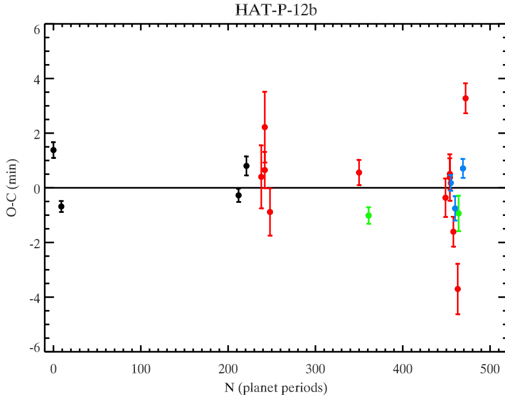
Figure 2. The difference between the best fit transit times and the observed transit times for HAT-P-12b. The black symbols represent transit timings from the discovery paper for this planet (Hartman et al. 2009). Also included are timings from the Exoplanet Transit Database (ETD; http://var2.astro.cz/ETD/ ) compiled by Lee et al. (2012; red symbols), and the measurements made by Lee et al. (2012; blue) and Sada et al. (2012; green). The horizontal axis shows the number of periods after the T_0 transit. We do not see any obvious correlation in the residuals that may suggest a transit timing variation, and hence the presence of an additional companion in the system. On the other hand, the number of outliers on this plot may imply that the timing uncertainties in some of these studies are underestimated.
