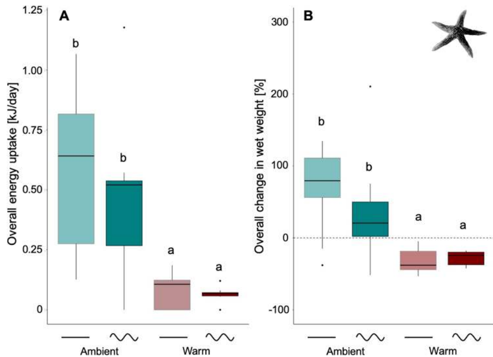
Figure 2. Energy uptake and change in wet weight of Asterias rubens . Energy uptake (A) and change in wet weight (B) during 72 days of experimentation, under ambient or warm and ‘constant’ or sinusoidal fluctuating temperature conditions (sum over the entire period, climate change in Fig. 1A). Data are presented as boxplots (median, upper and lower quartile (75 th and 25 th percentile), whiskers (1.5 times the interquartile range, outliers; N = 9). Significant differences between single treatment combinations were identified using a post hoc Tukey test at p < 0.05 and are indicated by lower-case letters.
