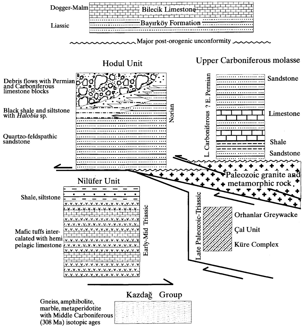
Fig. 4. Tectonostratigraphy of the pre-Jurassic units in the Sakarya Zone.
