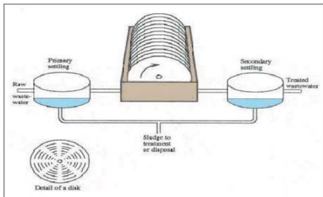
Figure 6. Diagram of an RBC unit 19 .
