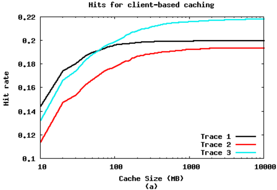
Figure 5. Overall sum of cache hits based on the local cache size
