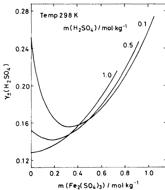
Fig. 4—Mean activity coefficients of H_2SO_4 in aqueous solutions of H_2SO_4 - Fe_2(SO_4)_3 , calculated by the McKay-Perring method.
