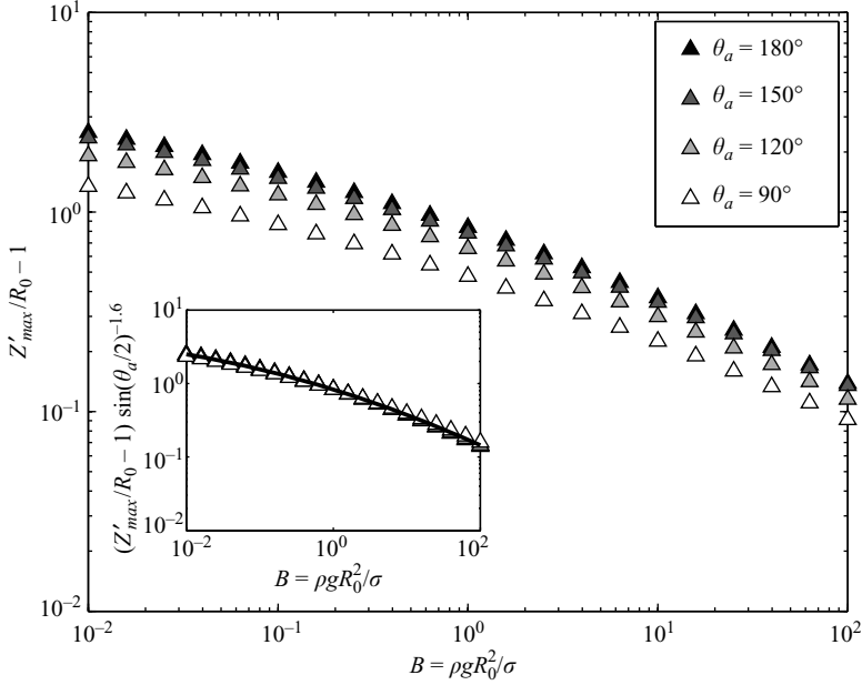
FIGURE 15. Penetration depth for a W \ll 1 impact. Theoretically predicted dependence of the dimensionless penetration depth on B for four values of the advancing contact angle, \theta_a . Inset: data collapse showing that the solid curve, defined by (5.3), captures the dependence of the penetration depth on B and \theta_a .
