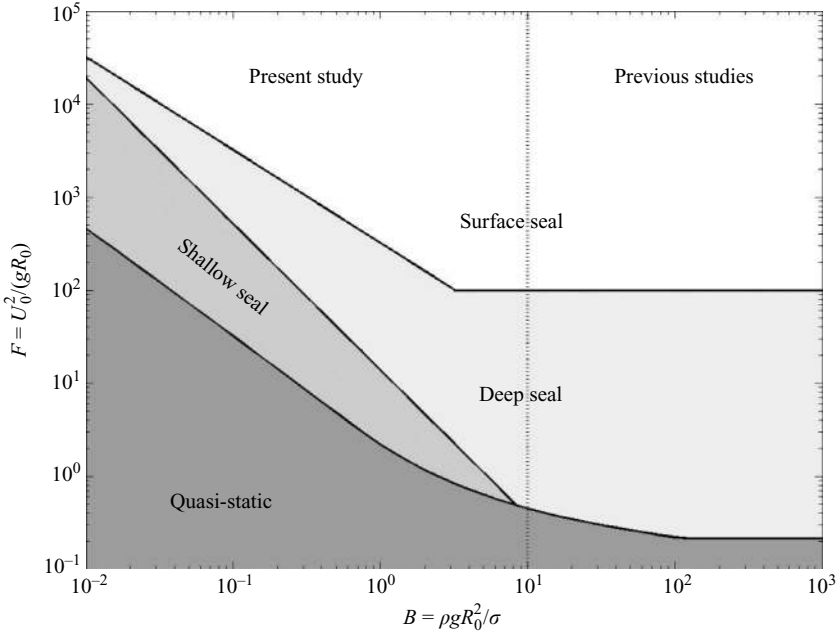
FIGURE 19. Regime diagram for the air–water entry of hydrophobic spheres, indicating the scope of the present study and observed cavity types (see §2). For all studies, Re \gg 1 , D > 1 , Q \gg 1 and \tilde{D} = 1.2 \times 10^{-3} . The theoretically predicted boundaries between the cavity regimes are given in §6, with the exception of the deep seal to surface seal boundary, given by the empirical fit W = 320 at low B (present study) and F = (1/6400)\tilde{D}^{-2} at high B (Birkhoff & Isaacs 1951). Note that cavitation is expected to arise at sufficiently high speed – specifically, when Q = (p - p_v)/(1/2 \rho U_0^2) < 1 , where p_v is the liquid vapour pressure.
