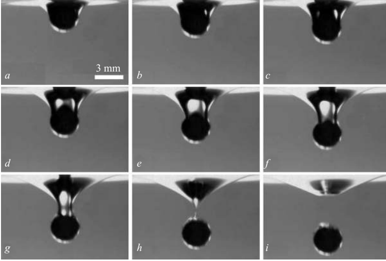
FIGURE 4. Quasi-static impact cavity. Video sequence of the water entry of a hydrophobic steel sphere at low B ( R_0=0.14 cm, \rho_s=7.7 g cm ^{-3} , U_0=30 cm s ^{-1} ). The time between successive images is 1.1 ms; W=1.9 ; B=0.27 .
