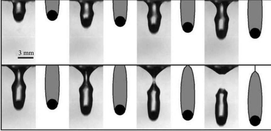
FIGURE 16. Zero B cavity model (6.4) alongside video sequence of shallow seal ( R_0 = 0.1 cm, \rho_s = 7.7 g cm ^{-3} , U_0 = 110 cm s ^{-1} ). The time between successive images is 1.1 ms; W = 17 ; B = 0.14 (experiment); B = 0 (model). Note that the model predicts pinch-off at the surface owing to the neglect of the longitudinal component of curvature.
