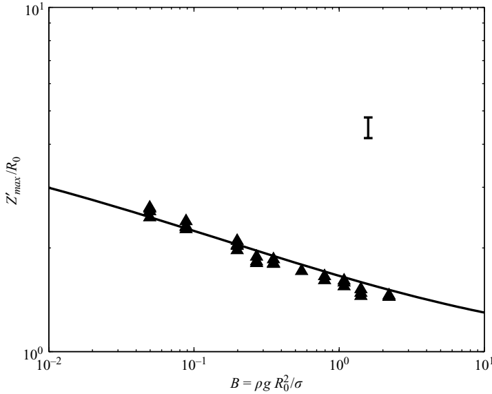
FIGURE 12. Penetration depth of a low speed ( W \ll 1 ) impactor with a quasi-static cavity. The triangles denote the experimental data for impacting spheres ( 10^{-4} < W < 10^{-2} ), and the solid curve is defined by (5.3) for \theta_a = 120^\circ , corresponding to the measured advancing contact angle. A characteristic error bar is shown.
