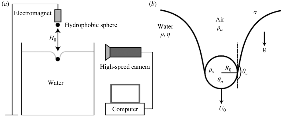
FIGURE 1. Schematic of (a) the experimental apparatus and (b) the impact parameters. The advancing contact angle is \theta_a , and the cavity cone angle is \theta_c .
