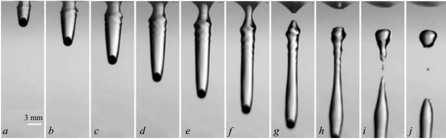
FIGURE 5. Shallow seal impact cavity. Video sequence of the water entry of a hydrophobic steel sphere at low B ( R_0=0.10 cm, \rho_s=7.7 g cm ^{-3} , U_0=230 cm s ^{-1} ). The time between successive images is 1.9 ms; W=72 ; B=0.14 .
