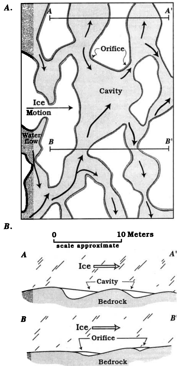
Figure 14. Idealized subglacial cavity network in (a) plan view and (b) cross section [after Kamb, 1987 ]. Unshaded areas are regions of ice-rock contact; shaded areas are regions of ice-rock separation (cavities). Flow directions in the cavities are indicated by arrows. Orifices are the most constricted parts of the cavity network and account for most of the energy losses.
