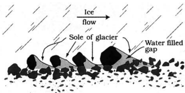
Figure 20. Hypothetical microcavity network at the ice-till interface. Small cavities may form at the lee of relatively large clasts that protrude above the mean surface of the till into the flowing ice.
