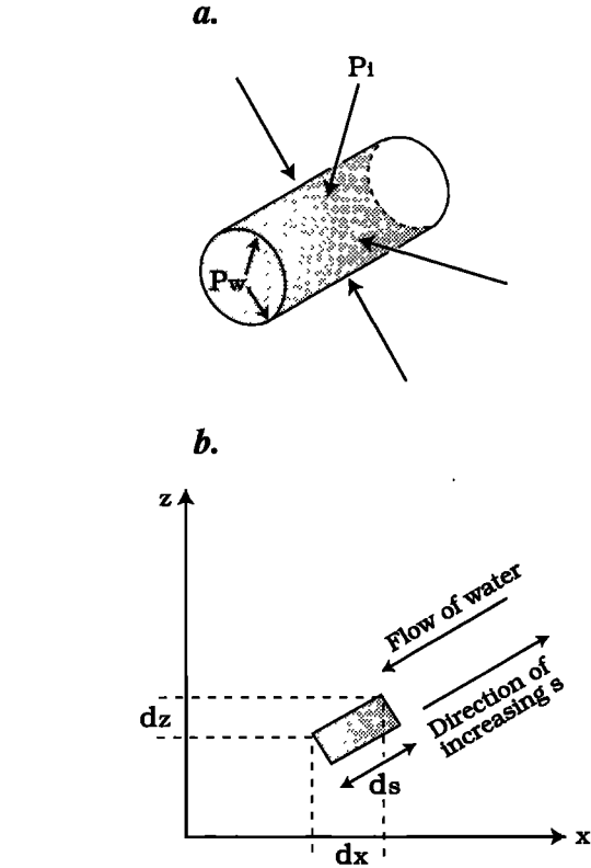
Figure 12. Schematic of a Röthlisberger channel [after Röthlisberger, 1972]. (a) The channel tends to close by creep of ice at overburden pressure p_i , but tends to be opened by melting as the flowing water (pressure p_w ) dissipates energy. (b) In general, the channel is inclined at some angle to the horizontal (the x axis). Reprinted from the Journal of Glaciology with permission of the International Glaciological Society.
