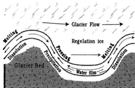
Figure 15. Regelation film of water at the ice-rock interface.
