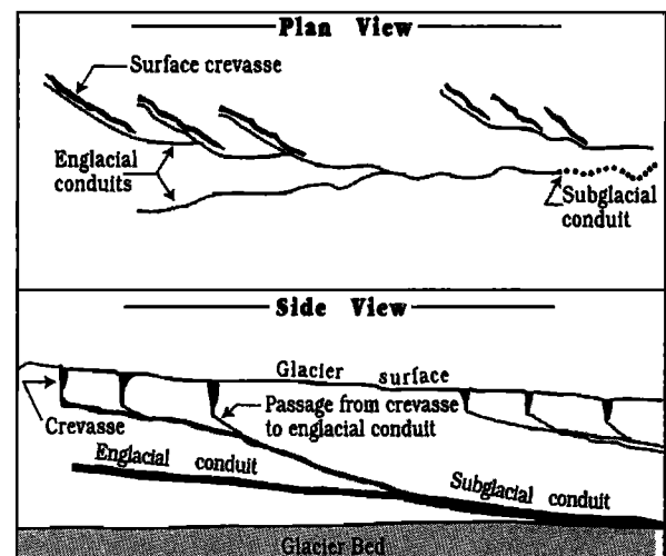
Figure 9. Geometry of hypothetical englacial drainage system, comprising both gently plunging conduits spawned by crevasse-bottom streams and steeply plunging “Shrevian” conduits formed where water exploits veins in the ice.
