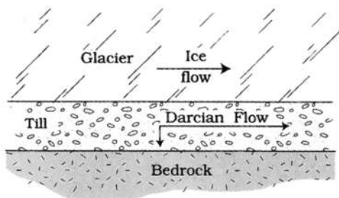
Figure 18. Drainage through subglacial till. Beneath most temperate alpine glaciers a thin layer of unconsolidated till lies between the base of the glacier and the underlying bedrock.
