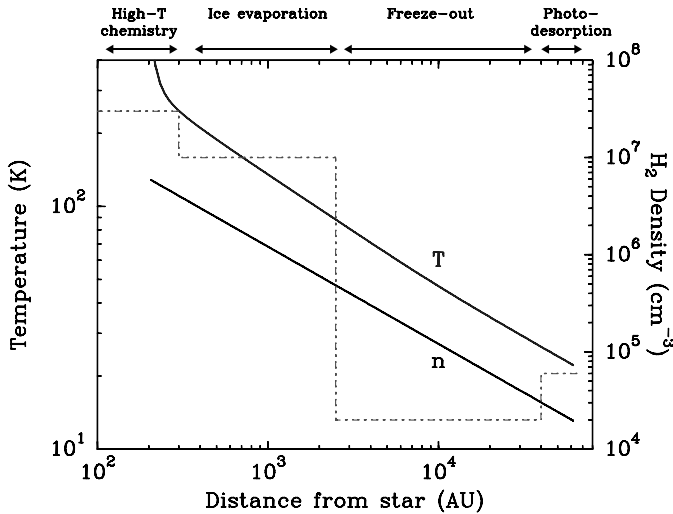
Fig. 2.—Temperature and density structure of a high-mass protostellar envelope. For illustrative purposes, a typical abundance profile is included (dash-dotted line) on an arbitrary scale, with the relevant chemical processes in each regime indicated at the top of the figure. The figure is based on the model of AFGL 2591 ( L = 6 \times 10^4 L_{\odot} ) presented by van der Tak et al. (1999). For distances of \sim 1 kpc, the typical Herschel beam of 20'' corresponds to 20,000 AU; i.e., it encompasses the entire envelope. For low-mass protostars, the ice evaporation zone moves inward to radii typically less than 100 AU. See the electronic edition of the PASP for a color version of this figure.
