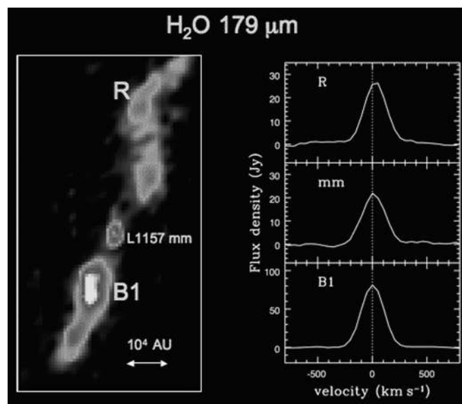
FIG. 9.— Herschel -PACS image of the \text{H}_2\text{O} 179\ \mu\text{m} line toward the stage 0 protostar L 1157, together with (spectrally unresolved) PACS spectra at three positions. The water emission is most significant in hot spots along the outflow where the (rotating) jet interacts directly with the cloud, as well as toward the protostar itself (based on Nisini et al. 2010). See the electronic edition of the PASP for a color version of this figure.
