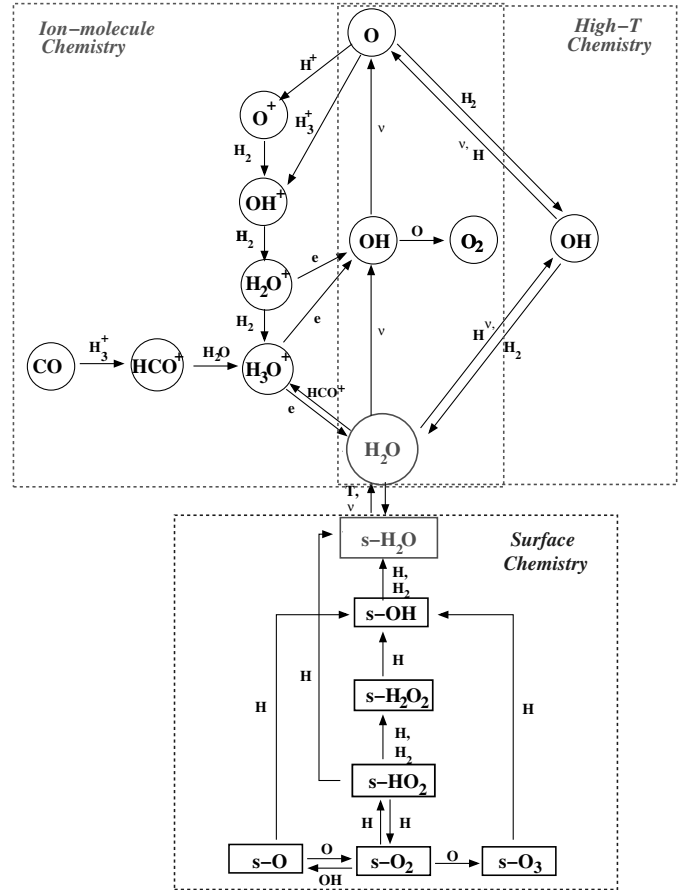
Fig. 3.—Summary of the main gas-phase and solid-state chemical reactions leading to the formation and destruction of \text{H}_2\text{O} . Three different chemical regimes can be distinguished: (1) ion-molecule chemistry, which dominates gas-phase chemistry at low T ; (2) high-temperature neutral-neutral chemistry; and (3) solid-state chemistry. The latter chemical scheme is based on the latest laboratory data by Ioppolo et al. (2010); s\text{-}X denotes species X on the ice surfaces. See the electronic edition of the PASP for a color version of this figure.
