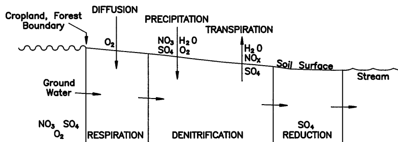
Figure 8. Conceptual model of below-ground processes affecting groundwater nutrients in riparian forest.
