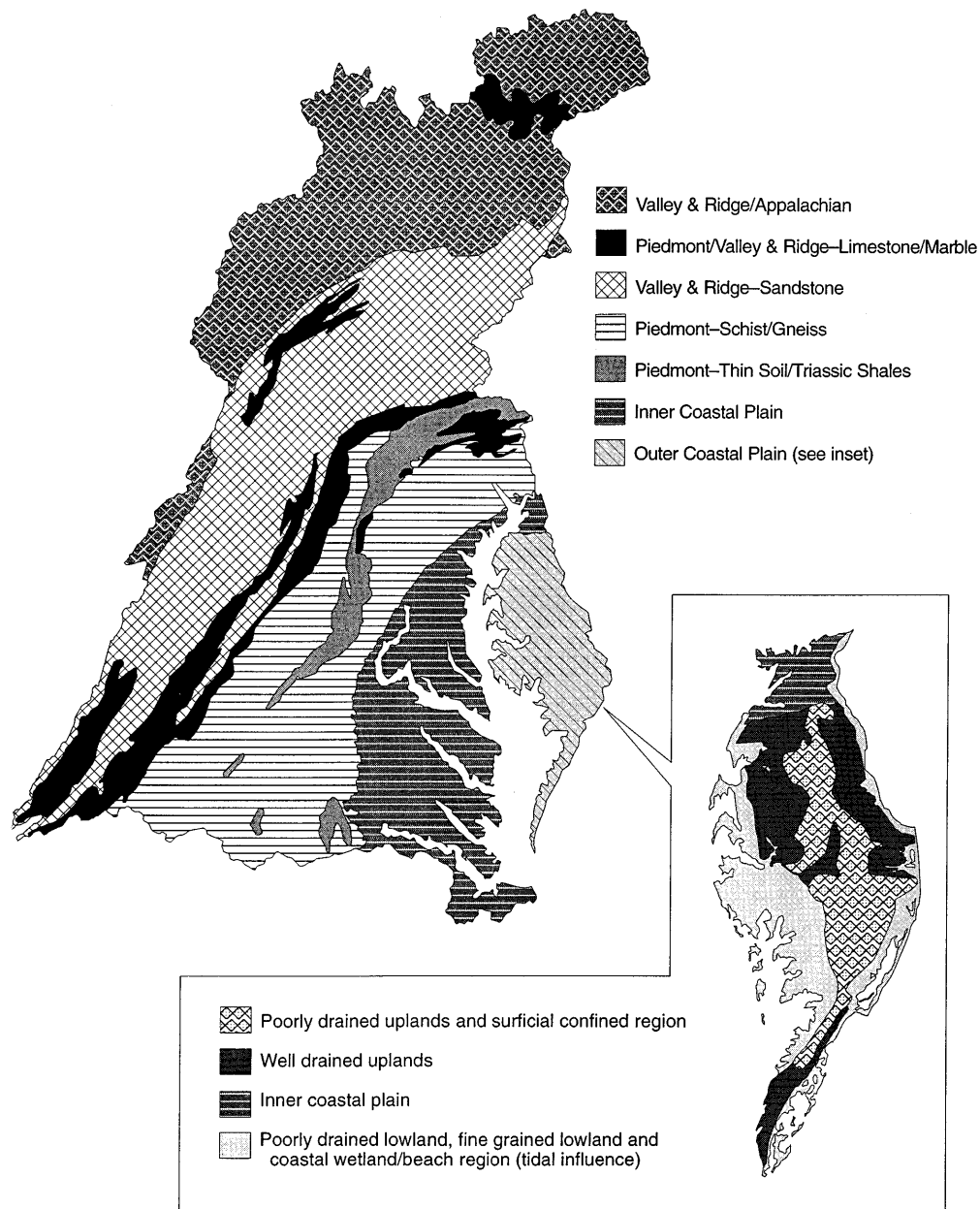
Figure 2. Physiographic regions of the Chesapeake Bay Watershed and hydrogeomorphic regions of the Delmarva Peninsula.
