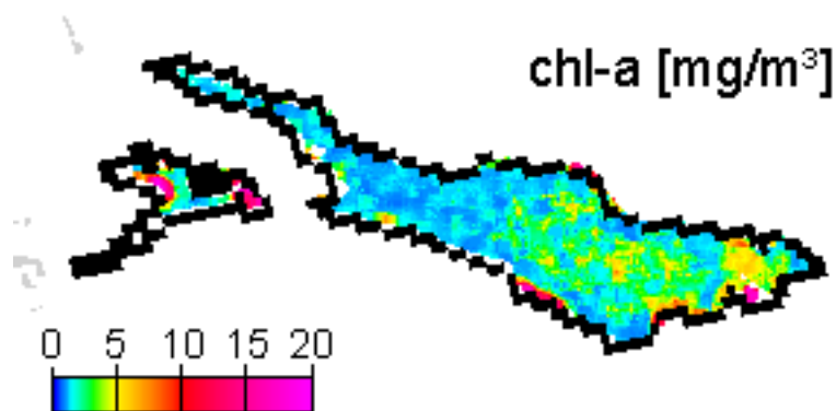
Figure 8. Chl-a concentration map for 15 April 2005.
