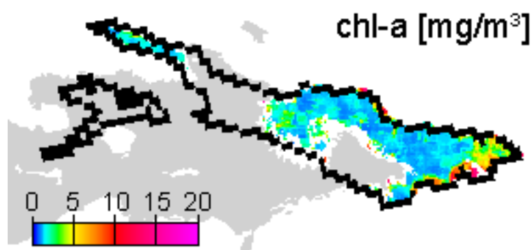
Figure 11. Chl-a and sm concentration maps for 2 November 2006. Pink and dark blue color represent threshold concentrations allowed by the algorithm, which indicates erroneous processing.
