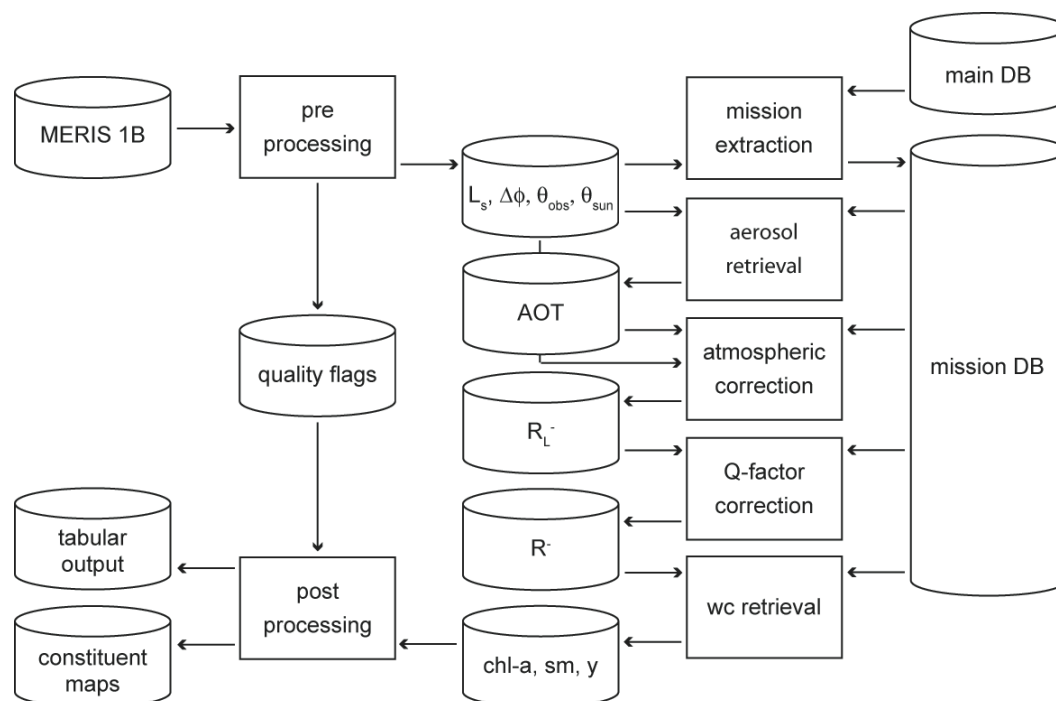
Figure 3. Flow chart of the automatic data processing chain. The mission DB contains the LUTs for atmospheric and Q-factor correction, for the data specifications defined in the mission extraction. The tabular output contains concentration and retrieval quality parameters for FU and lake means.
