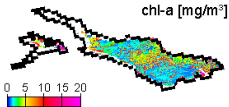
Figure 5. Chl-a, sm and y map for 20 April 2007, after application of the selective filter.
