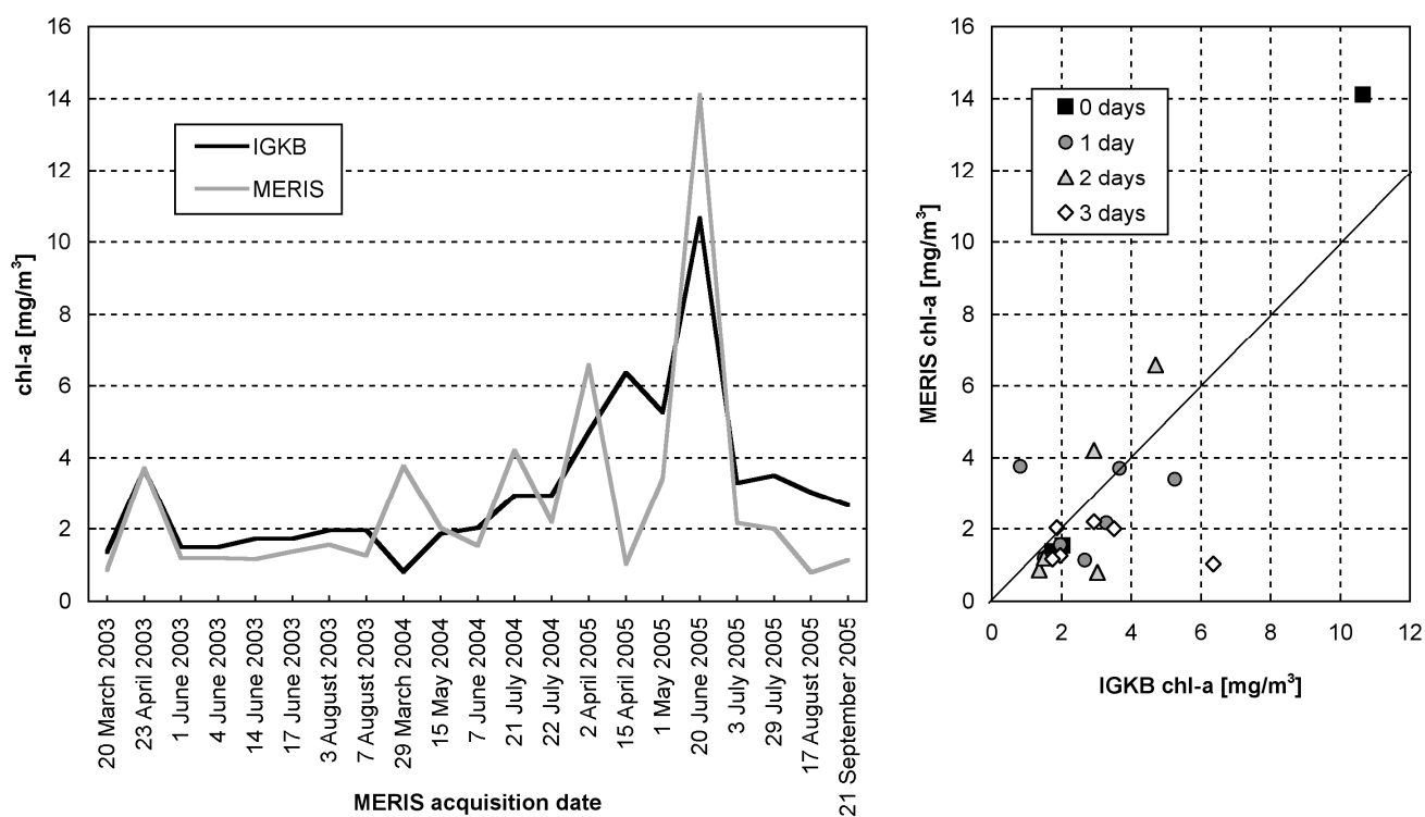
Figure 7. 21 chl-a data pairs for the site FU, 2003-2005. The number of days between data acquisition are indicated in the figure on the right. MERIS values are filtered outputs, as shown in Figure 5 .
