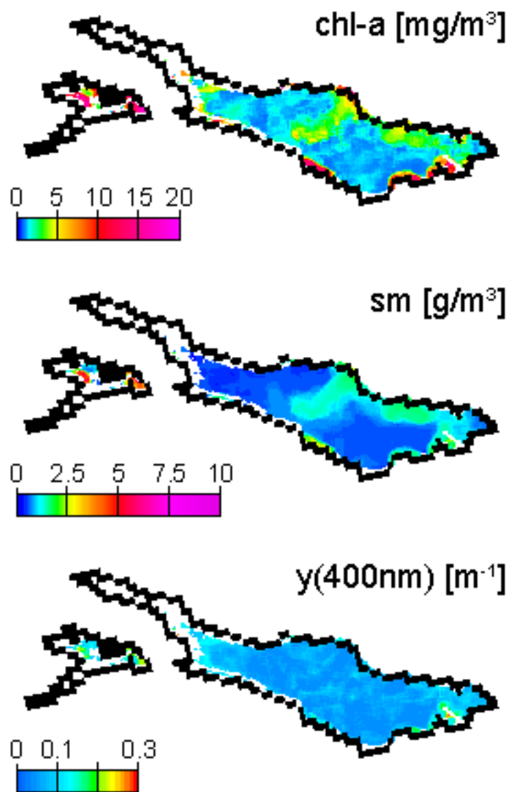
Figure 5. Chl-a, sm and y map for 20 April 2007, after application of the selective filter.
