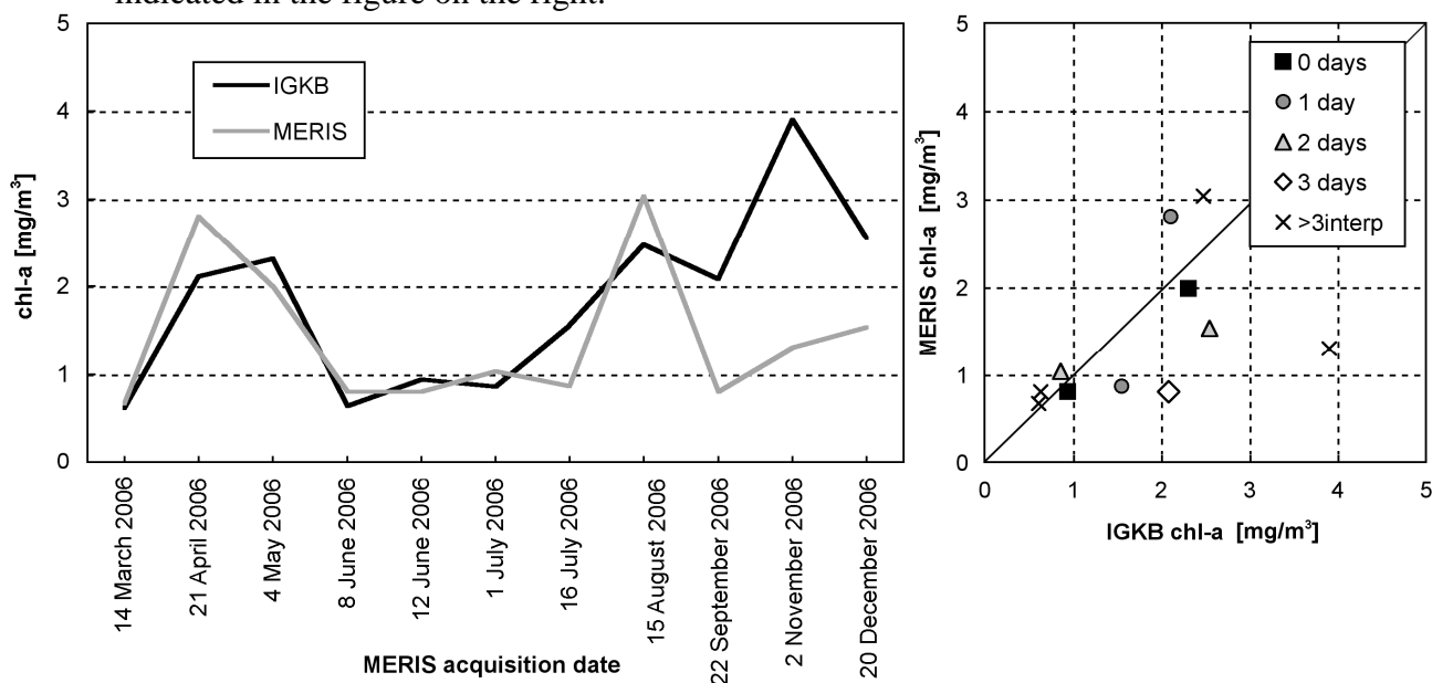
Figure 9. 11 chl-a data pairs for validation of IGKB and MERIS measurements, for the site FU, 2006. Number of days between in situ sampling and satellite overpass are indicated in the figure on the right.
