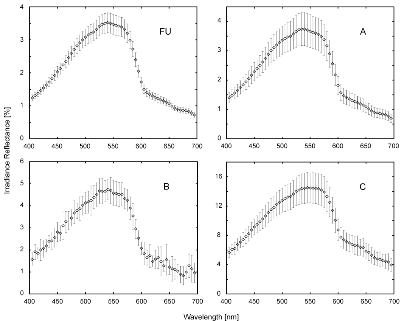
Figure 2. RAMSES data acquired in the sites FU and A-C ( Figure 1 ) at a depth of 20 cm, on 20 April 2007.
