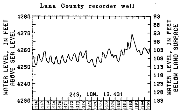
Figure 2.--Ground-water levels for the last 20 years or period of record.
