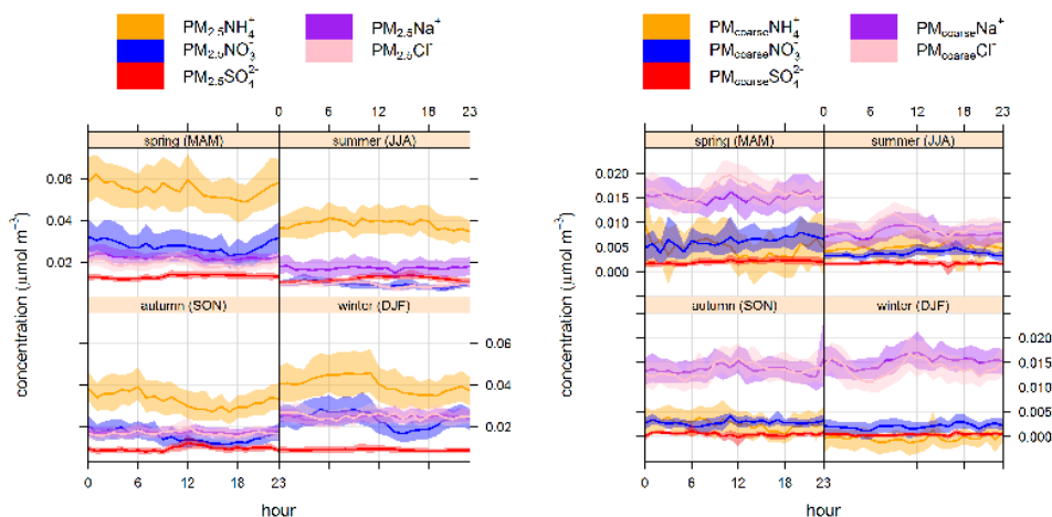
Figure 3. Median seasonal diurnal cycles of molar concentrations of PM 2.5 and PM coarse , NH 4 + , NO 3 - , SO 4 2- , Na + and Cl - using data from January 2007 to December 2012, with the shading showing the 95 % confidence level of the median. (Graphs produced using Open air; Carslaw and Ropkins, 2012).
