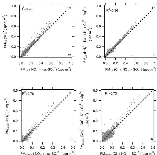
Figure 4. Measured ion balance for the year 2012 in microequivalents per cubic metre. (a) Neutralisation of PM 2.5 NH 4 + by PM 2.5 nss-SO 4 2- and PM 2.5 NO 3 - , (b) ion balance of measured PM 2.5 anions (Cl - , NO 3 - and SO 4 2- ) and measured PM 2.5 cations (NH 4 + , Na + , K + , Ca 2+ and Mg 2+ ), (c) neutralisation of PM coarse NH 4 + by PM coarse nss-SO 4 2- and PM coarse NO 3 - , (d) ion balance of measured PM coarse anions (Cl - , NO 3 - and SO 4 2- ) and measured PM coarse cations (NH 4 + , Na + , K + , Ca 2+ and Mg 2+ ).
