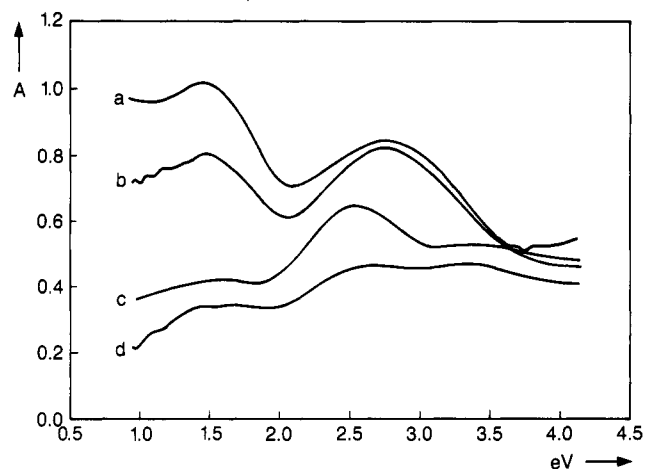
Figure 7. Absorption spectra of poly(3-butylsulfonate pyrrole) 16: (a) as a heavily doped film on ITO glass electrode; (b) the same film of a dissolved in water; (c) as purposely dedoped film on ITO glass electrode; (d) the same film of c dissolved in water.
