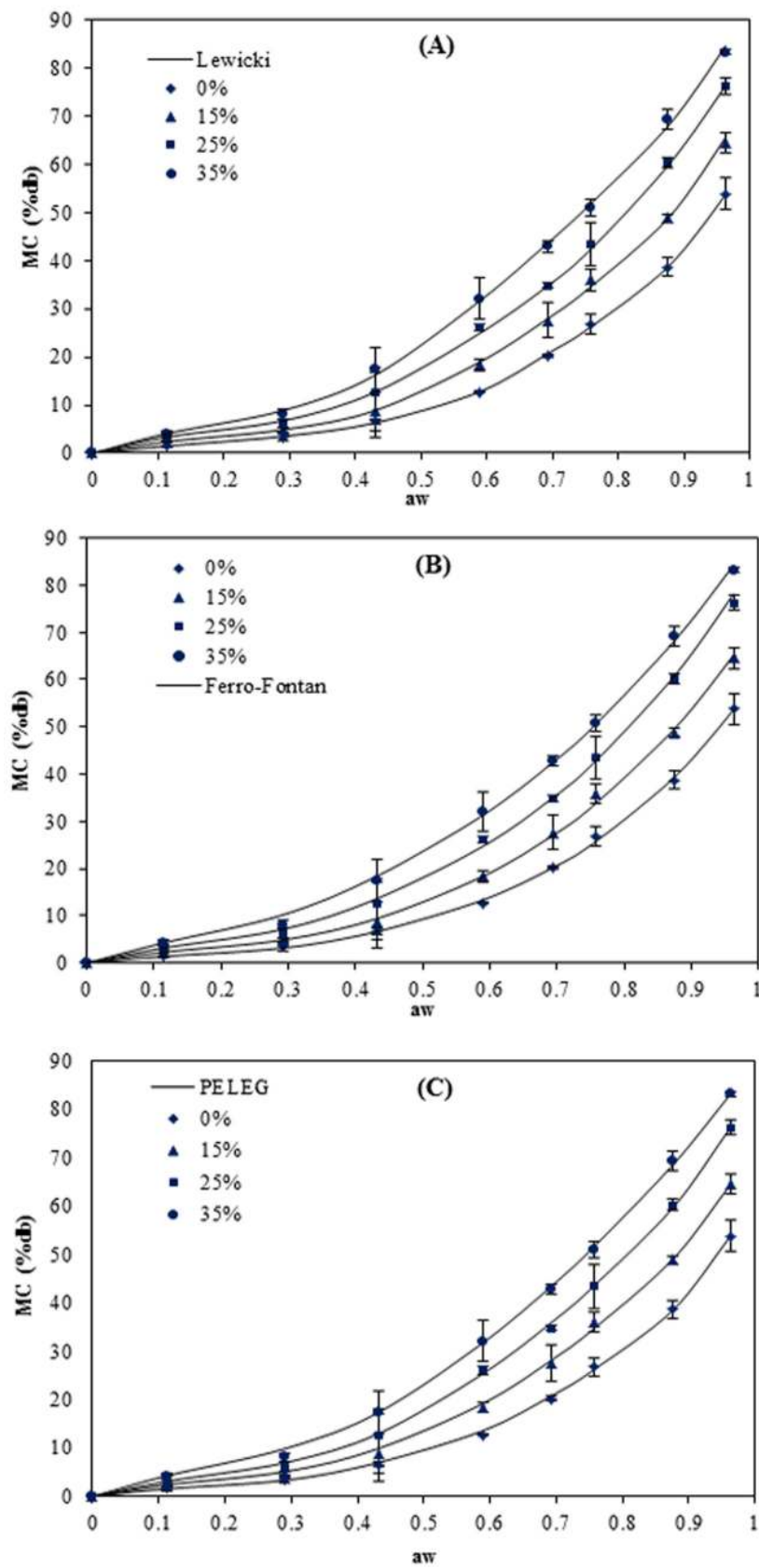
Figure 1. Equilibrium moisture sorption isotherm of pea starch film with different glycerol content ( w/w ) at 5 °C. The symbols are experimental data and the lines are from the equations obtained by fitting the experimental data to Lewicki (A), Ferro-Fontan (B) and PELEG (C) equations.
