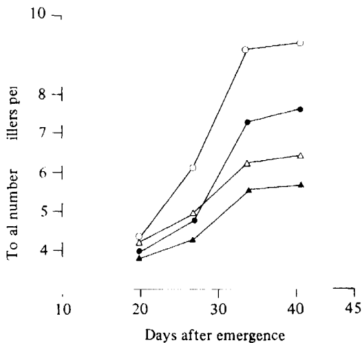
Fig. 2. Total number of tillers per plant in photoperiod and water stress treatments in 1980. \Delta , ND irrigated; \circ , LD irrigated; \blacktriangle , ND stress; \bullet , LD stress.
