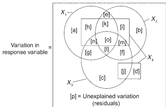
FIG. 5. Venn diagram representing partitioning the variation of a response variable or data table among four sets of explanatory (environmental and spatial) variables ( X_1 , X_2 , X_3 , X_4 ). The rectangles represent 100% of the variation in the response variable (Legendre 1993).
