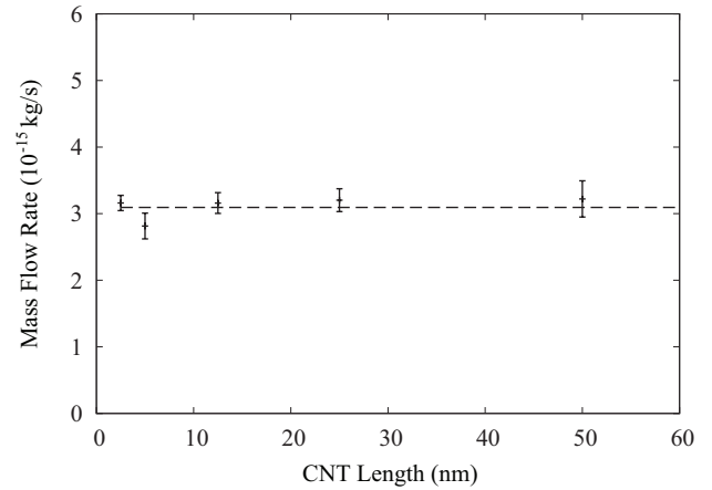
Fig. 4: Relationship between mass flow rate and CNT length under a 200 MPa pressure difference. The horizontal dashed line indicates an average mass flow rate of 3.11 \times 10^{-15} kg/s.
