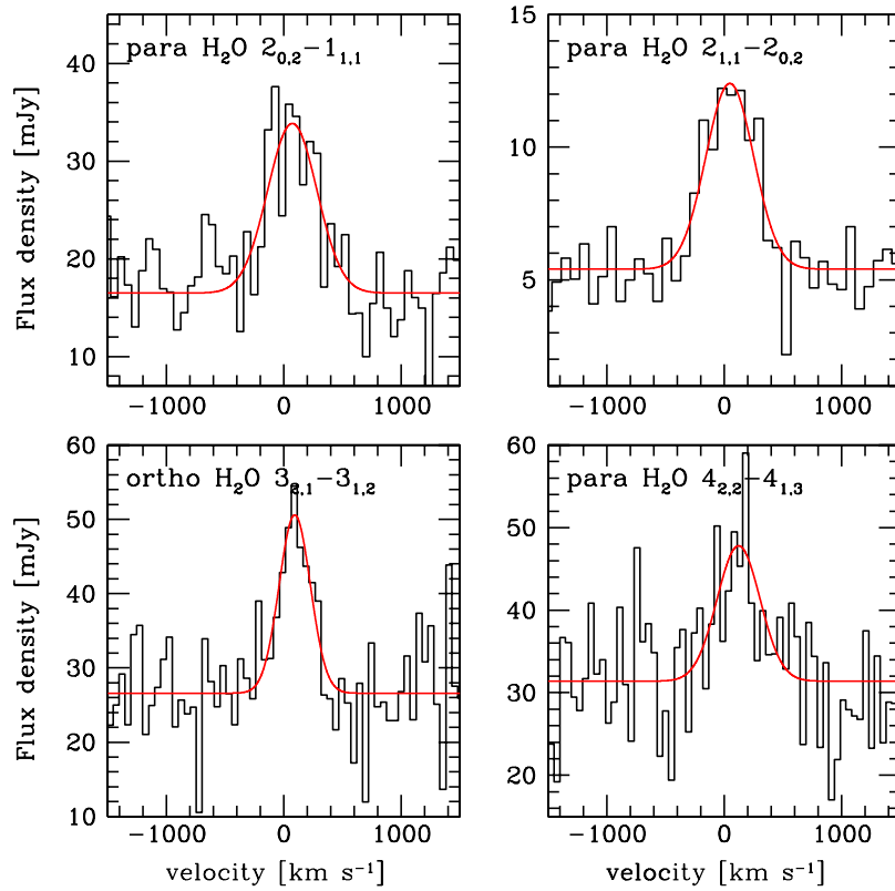
Figure 2. Spectra of H 2 O emission lines from APM08279+5255 at a common frequency resolution of 40 MHz. The horizontal axis shows velocity relative to redshift z = 3.911 . The red curves indicate Gaussian fits to each spectrum.
