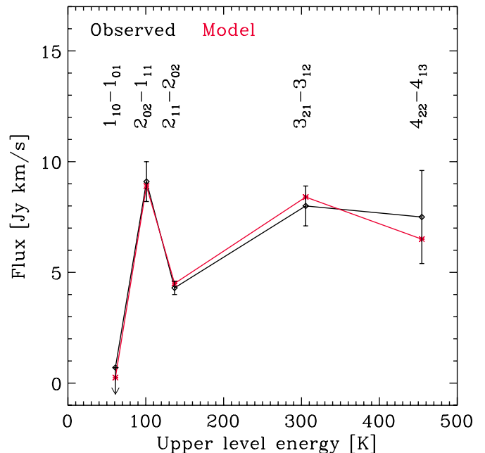
Figure 3. Flux in H 2 O emission lines from APM08279+5255 as a function of upper level energy E_u . Black symbols and error bars indicate the observed line fluxes and the previously published upper limit on 1_{1,0} - 1_{0,1} (indicated by a downward arrow). Red crosses indicate values produced by our model as described in the text.
