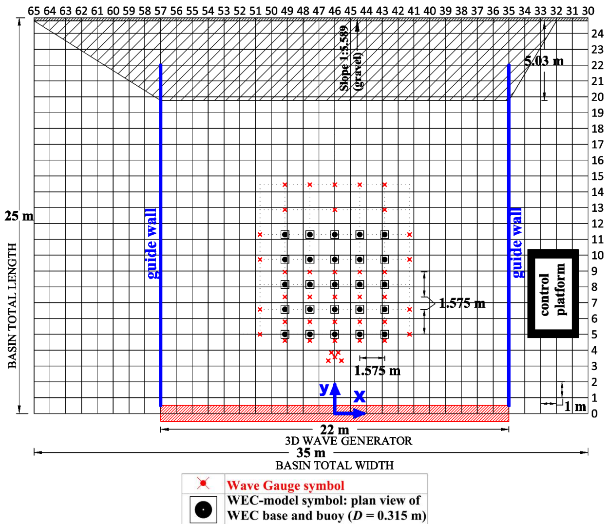
Figure 4. Plan view of the WECwakes experimental arrangement in the DHI wave basin and 5 × 5-WEC rectilinear array. Grid at 1.0 m increments, wave gauge arrangement (x) and WEC positions (●) are indicated. The hatched region along the x-axis at the bottom of the figure denotes the extent of the wave paddles, while at the opposite end the wave absorbing beach is shown. At the sides, plywood guide walls are used. Water depth is constant, d_w = 0.70 m.
