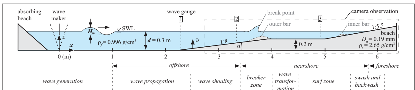
FIGURE 2 | Side view of the experimental set-up with wave maker, ultra-sonic wave gauge location, reference bed profile ( t = 0 h), and camera observation section.
