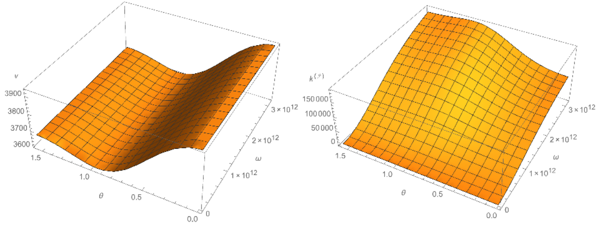
Fig. 5 LS-model, qP wave: phase velocity v and attenuation factor k^{(3)} vs the propagation angle \theta and the angular frequency \omega . Relaxation time t_0 = 1 \times 10^{-12} s.
