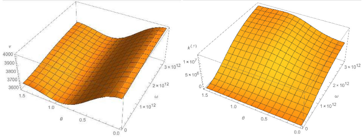
Fig. 8 GL-model, qP wave: phase velocity v and attenuation factor k^{(3)} vs the propagation angle \theta and the angular frequency \omega . Relaxation times t_0 = 1 \times 10^{-12} s and t_1 = 40 t_0 .
