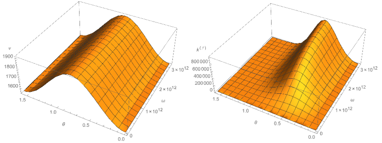
Fig. 9 GL-model, qS wave: phase velocity v and attenuation factor k^{(3)} vs the propagation angle \theta and the angular frequency \omega . Relaxation times t_0 = 1 \times 10^{-12} s and t_1 = 40 t_0 .
