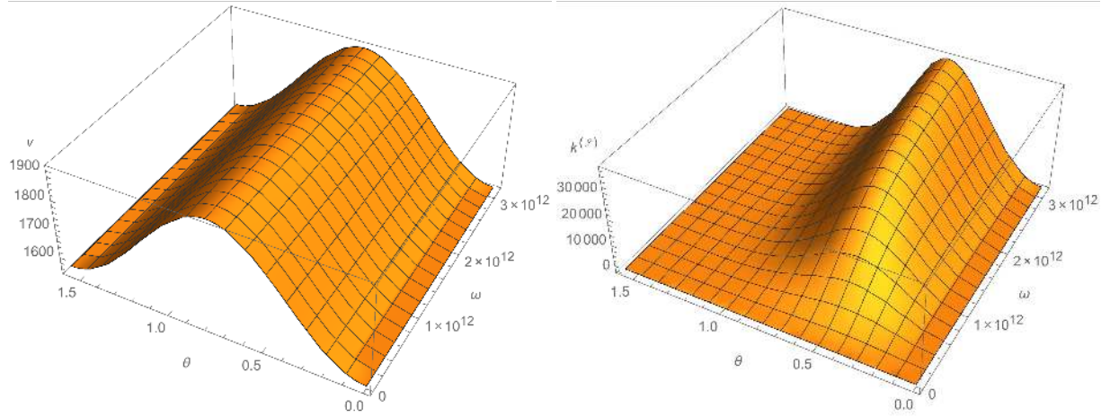
Fig. 6 LS-model, qS wave: phase velocity v and attenuation factor k^{(3)} vs the propagation angle \theta and the angular frequency \omega . Relaxation time t_0 = 1 \times 10^{-12} s.
