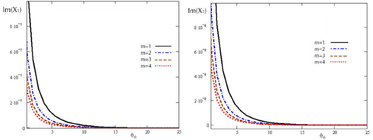
Fig. 16 LS-model: imaginary parts of the reflection coefficients X_1 and X_2 versus \theta_0 for different values of the relaxation time t_0 = m \times 10^{-12} s.
