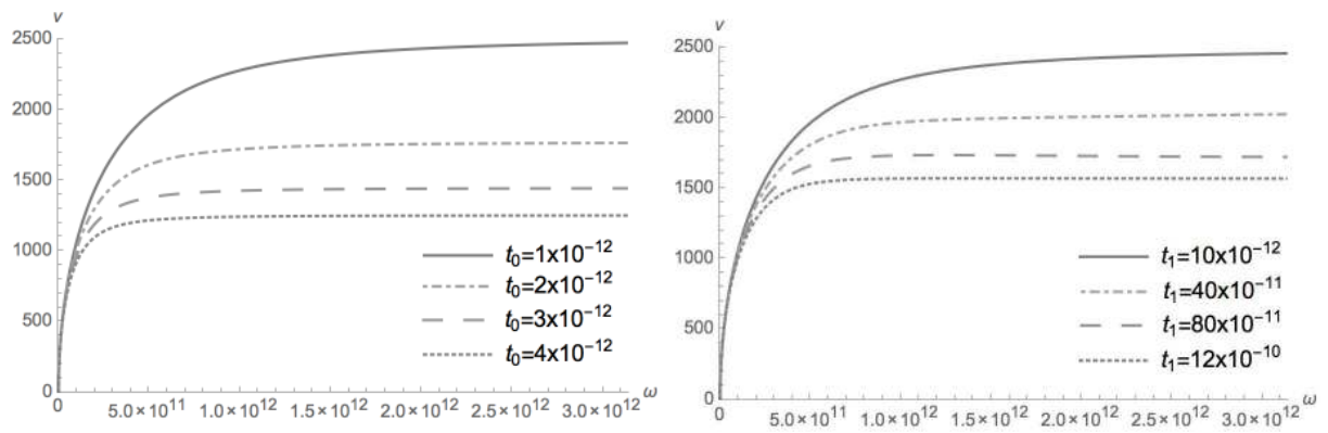
Fig. 12 Parametric analysis of phase velocities v : LS-model (left) for various values of relaxation time t_0 and GL-model (right) for t_0 = 1 \times 10^{-12} s and various values of t_1 .
