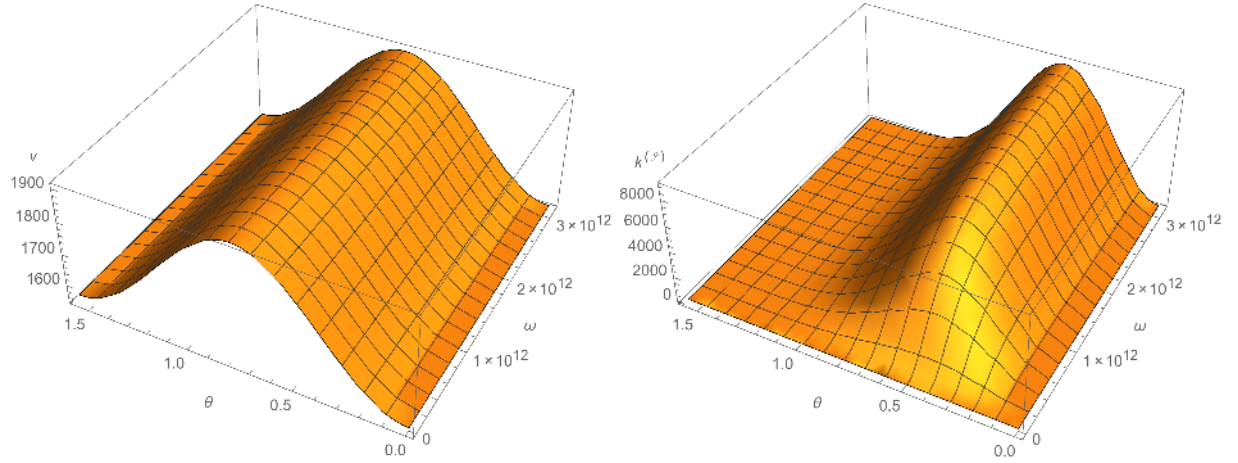
Fig. 3 CD-model, qS wave: phase velocity v and attenuation factor k^{(3)} vs the propagation angle \theta and the angular frequency \omega .
