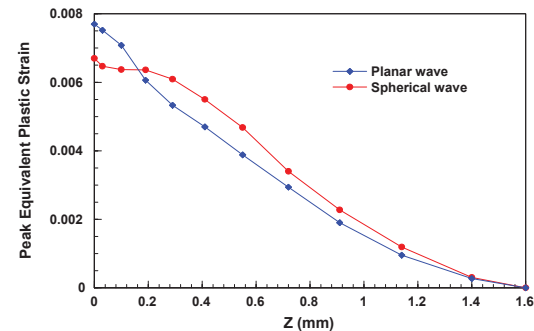
Fig. 11 The calculated peak equivalent plastic strain along the thickness of the copper plate.
