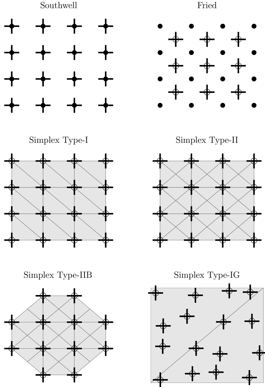
Fig. 3: Southwell geometry (top left) and Fried (top right) sensor geometries compared with 4 different SABRE geometries (middle and bottom rows). Black dots are the phase point locations, horizontal and vertical lines are the slope measurements in the x and y directions, respectively. The open circles are the locations of the slope measurements. Gray lines in the SABRE geometries are the triangle edges, while the shaded area inside the triangulations is the area in which \phi(x, y) is defined.
