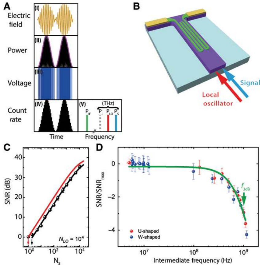
Figure 9: Heterodyne mixing with SNSPDs.
