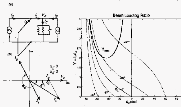
Figure 6: Equivalent circuit (a) with stub line matching and the phasors (b) including the stub line current. Beam loading limit (right) as a function of impedance angle and loading angle.
