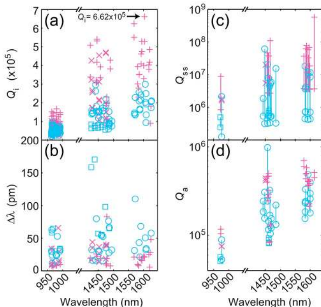
FIG. 2. (Color online) Measured (a) Q_i and (b) \Delta\lambda for the (+, \times ) GaAs TE and TM-polarized microdisk modes and ( \circ , \square ) \text{Al}_{0.18}\text{Ga}_{0.82}\text{As} TE and TM modes, respectively. In (c) and (d), connected points represent calculated bounds on (c) Q_{\text{ss}} and (d) Q_a for each family of modes. The data were compiled from two disks of each material.
