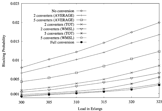
Fig. 9. Blocking probability versus traffic load in EON using LLR-FF algorithm.
