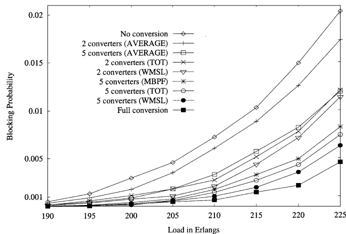
Fig. 8. Blocking probability versus traffic load in NSFNET using LLR-FF algorithm.
