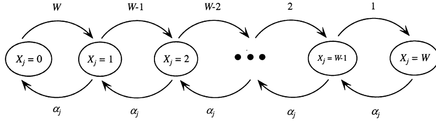
Fig. 2. Markov chain for free wavelength distribution on link j .
