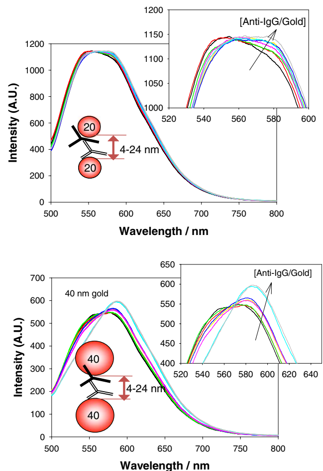
Fig. 3 Scattering spectra (also includes transmitted light) of gold colloid-coated HTS wells before and after the immunoassay is completed. Top anti-IgG-modified 20 nm gold (0.05, 0.01, 0.5, 5, 10, and 15 \mu\text{g/mL} in the direction of the arrow) Bottom anti-IgG-modified 40 nm gold (0.01, 0.05, 0.1, 1, 5, and 10 \mu\text{g/mL} in the direction of the arrow). The arrow indicates the increase in concentration of anti-IgG-modified gold colloids used as the detector antibody
