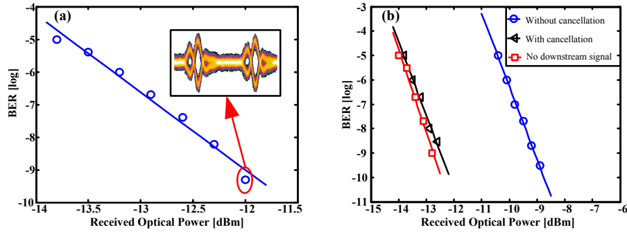
Fig. 4. (a) Measurement results of the downstream signal. (b) BER result of the upstream signal.
