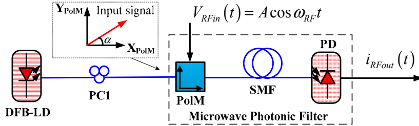
Fig. 2. PM-IM conversion in a SMF link.
