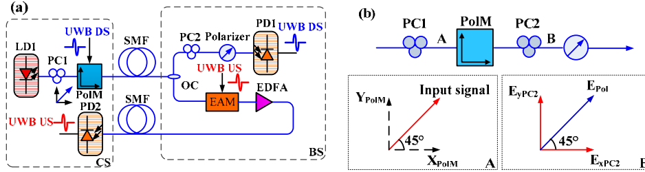
Fig. 1. (a) A bidirectional UWB optical fiber system with wavelength reuse for upstream transmission. (b) Equivalent MZM using a PolM, a PC and a polarizer.
