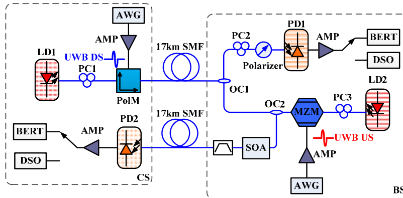
Fig. 3. Experimental setup. LD: laser-diode, PC: polarization controller, PolM: polarization modulator, AWG: arbitrary waveform generator, AMP: electrical amplifier, PD: photodiode, BERT: bit error rate tester, DSO: digital storage oscilloscope, MZM: Mach-Zehnder modulator, SOA: semiconductor optical amplifier
