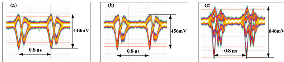
Fig. 5. Eye diagrams of the upstream signal. (a) Without downstream transmission, (b) with chromatic dispersion cancellation, and (c) without chromatic dispersion cancellation.
