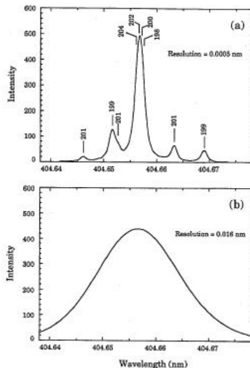
Fig. 2. (a) Spectrum of the 404.6-nm line of natural Hg from a pencil-type lamp at an instrumental resolution of 0.03\text{ cm}^{-1} ( 0.0005\text{ nm} ). (b) The same spectrum with the resolution degraded to 1.0\text{ cm}^{-1} ( 0.016\text{ nm} ) by convolution with a Gaussian instrumental function.
