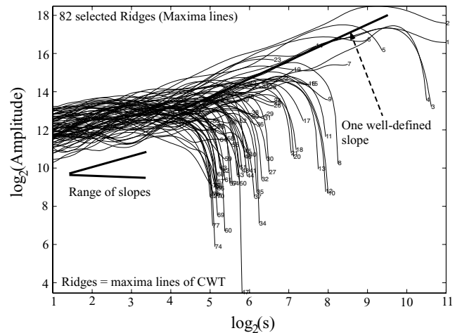
Figure 10. Logarithmic plot of the amplitude of CWT along ridges (maxima lines of the continuous wavelet transform ) in the case of the ‘Kobe sequence’. At large scales there is only one well-defined, predominant slope of the lines, while at smaller scales there is a range of slopes. Because of the large number of WTMM lines, only a representative set was considered in this plot.
