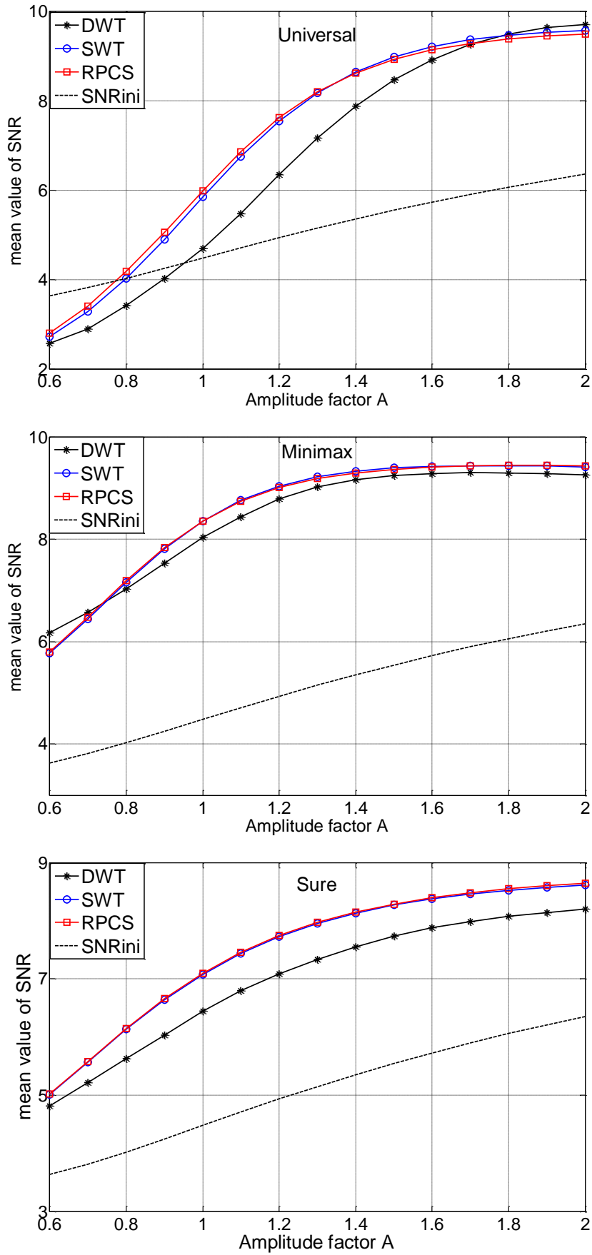
Figure 4 Mean values of the SNR after denoising of 1000 A-scans in each of the different sets for the different types of threshold selection
