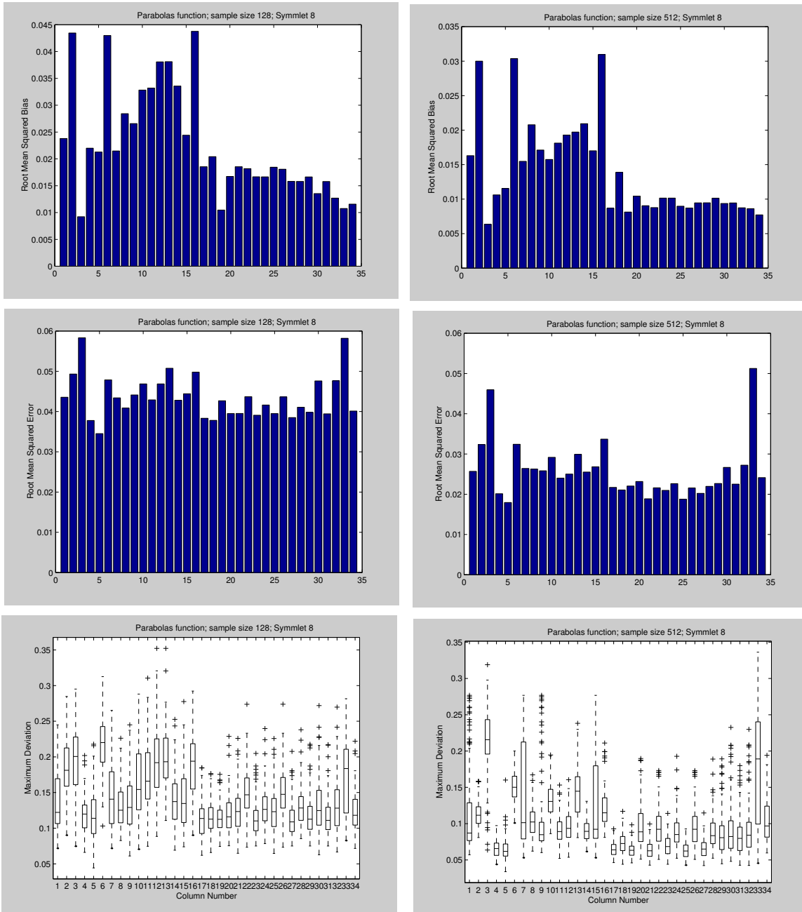
Figure 8.12: Performance of the estimators for the Parabol function over 100 simulations. The root signal-to-noise ratio is equal to 3 for sample sizes of 128 (left) and 512 (right) design points. The wavelet filter used is the Symmlet 8.
